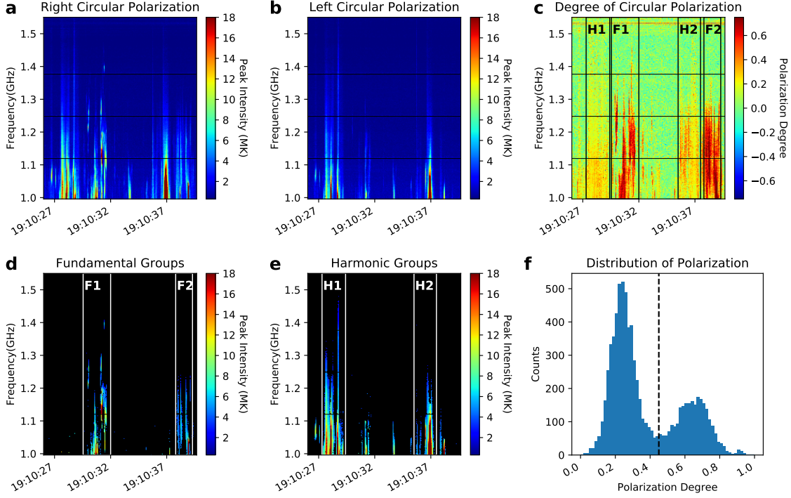
Figure 2. Polarization of the dm- \lambda type III bursts. (a, b) Dynamic spectrum of the observed dm- \lambda type III bursts in RCP and LCP, respectively, colored by their peak intensity I_{\text{pk}} in brightness temperature units. (c) Same as (a) and (b), but colored by their degree of circular polarization. (d, e) Fundamental (labeled “F1” and “F2”) and harmonic (labeled “H1” and “H2”) burst groups separated by their degree of polarization properties. They correspond respectively to the weakly and strongly polarized groups in the left and right portion of the histogram plot of (f) separated at degree of polarization level of 45% (vertical dashed line). Only bursts with SNR > 13 are shown in (d-f).
