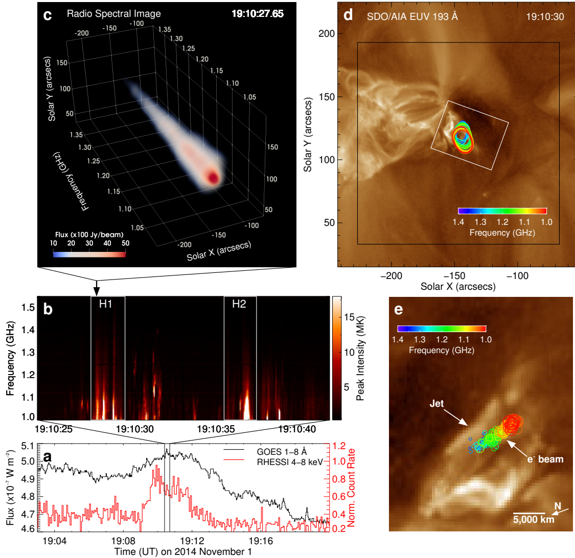
Figure 1. Radio bursts from fast electron beams. (a) Light curves of the solar jet event at two X-ray energies. (b) Spatially-resolved intensity of dm-λ type III radio bursts as a function of frequency and time I_{\text{pk}}(\nu, t) , or “vector dynamic spectrum”, recorded by the VLA around the X-ray peak. (c) Volume rendering of a 3D spectral image cube of an example radio burst made at 200 independent frequency channels within a single 50-ms integration at 19:10:27.65 UT (black arrow indicates the time). (d) Contours of the same type III burst in panel (c) (85% of the maximum), each of which representing a radio image at a single frequency slice of the 3D spectral imaging cube colored from red to blue in increasing frequency. Background is SDO/AIA 193 Å EUV image (gold; showing coronal plasma at \sim 1.6 MK). Black box marks the field of view of (c). The ensemble of the image centroids is shown in an enlarged view (e) as colored circles (size scaled by their peak flux), delineating the trajectory of a fast electron beam propagating at an apparent speed of v_{bx}^{\text{app}} \gtrsim 0.5c in projection. The display region is marked as the white box in (d) rotated counter-clockwise by 110^\circ .
