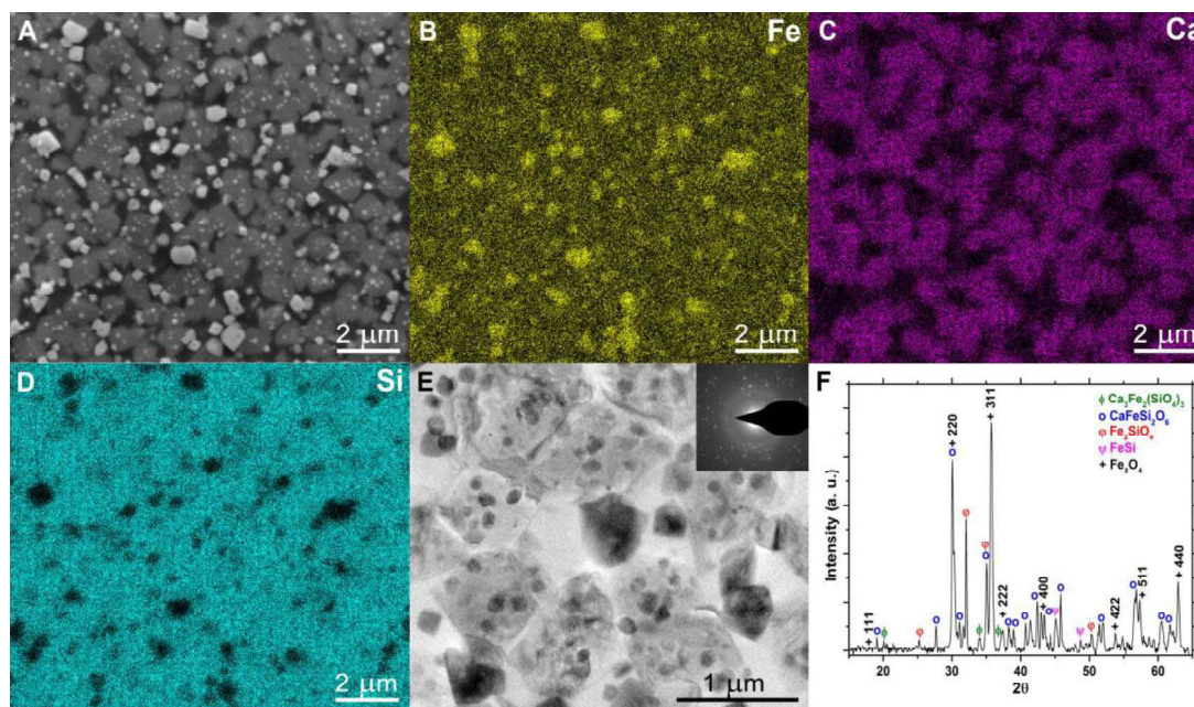
Figure 1. (A) BSE SEM image of the synthetic basalt; and (B-D) associated EDX chemical maps showing the elemental distribution of (B) iron; (C) calcium; and (D) silicon. (E) BF TEM image of the \text{Fe}_3\text{O}_4 grains within the silicate matrix ranging from \sim 50 to \sim 500 nm, with SAED (inset). (F) XRD pattern of the synthetic basalt, confirming the \text{Fe}_3\text{O}_4 phase (indexed, JCPDS 75-449), as well as the additional phases of \text{CaFeSi}_2\text{O}_6 , \text{Ca}_2\text{Fe}_2(\text{SiO}_4)_3 and \text{FeSi} .
