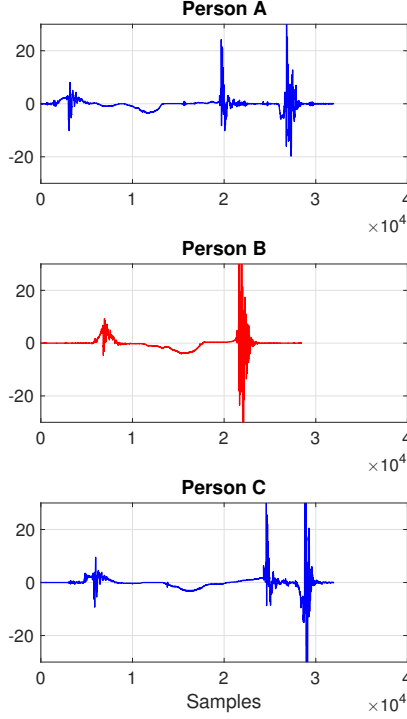
Fig. 8. Figure illustrates raw accelerometer signals of Persons A , Persons B , and C , when opening and closing a door. The signals depict high similarities between Person A and C , while Person B is relatively unique. Such uniqueness yields high classification accuracy for Person B with the door event type .
