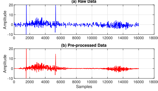
Fig. 3. We use spectral subtraction to increase the Signal-to-Noise Ratio (SNR). (a) depicts raw time-series gyroscope signal; and (b) depicts the resulting spectral subtraction.
