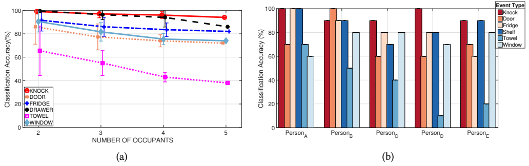
Fig. 6. Figure depicts classification accuracy by varying number of occupants of each event type (for known labels scenario). Each data point is an average accuracy of all combinations within each number of occupants. As the number of occupants increases, classification accuracy decreases. The average accuracy of different event types for five occupants case yields 74%. (b) Figure depicts classification accuracy due to different occupants. Certain pair of event types yield contradicting accuracy across different occupants. SenseTribute takes advantage of such phenomenon to amplify the final accuracy in its Ensemble Module .
