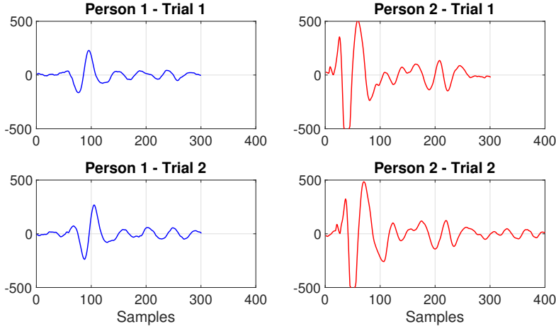
Fig. 14. Figure illustrates raw signals of footsteps from two participants captured by a geophone. The signals depict high correlation between trials from the same participant. However, the signals are sufficiently differentiable across the two participants due to differing gait movements.
