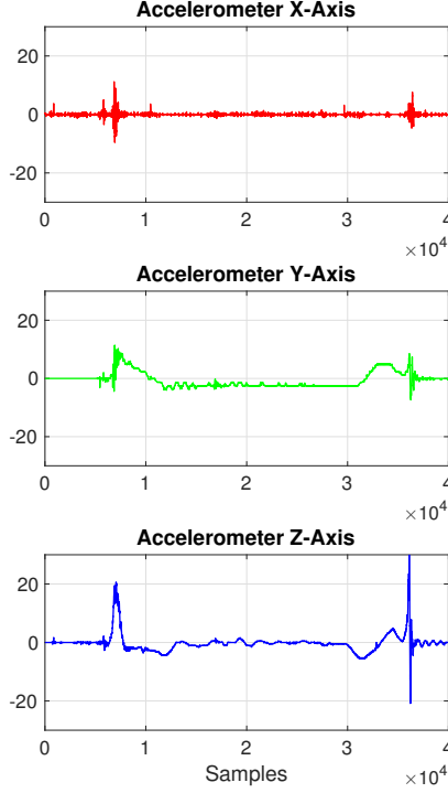
Fig. 13. Figure illustrates the raw accelerometer signals of X, Y, and Z-axes when a participant opens and closes a fridge door. Due to the orientation of accelerometer installed on the fridge door during the experiment (as described in Section 4.1.1), the Z-axis captures rich information content of the fridge door opening and closing motion, while the other two axes does not add additional information when classifying occupants.
