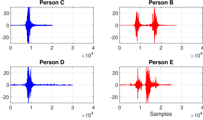
Fig. 7. Figure illustrates raw accelerometer signals of Persons B, C, D and E , when dispensing towel. The signals depict high similarities between Persons C and D , as well as Persons B and E . This can be possibly explained when considering similar physical built between the occupant pairs.
