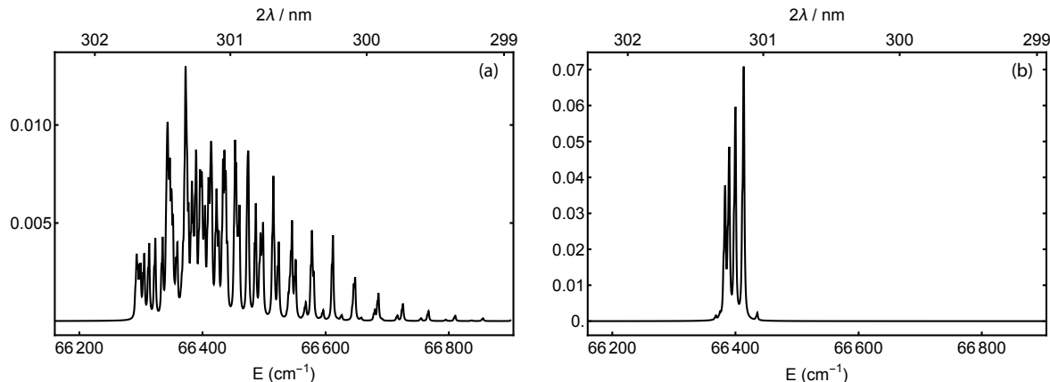
Figure 2. Calculated two-photon excitation spectra from the neutral ^{16}\text{O}_2 X^3\Sigma_g^- ground state to the d^1\Pi_g Rydberg state, both in their ground vibrational state. The temperatures shown correspond to (a) an effusive beam at 300 K or (b) a supersonically-expanded one at 5 K. The traces are normalized such that the sum of all transitions is one; note the resulting scale change.
