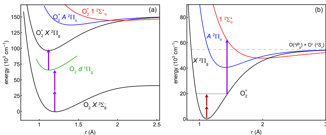
Figure 1. General scheme of the proposed experiments. (a) The ^{16}\text{O}_2^+ ion is prepared in its ground vibrational state by photoionization through the neutral d^1\Pi_g Rydberg state with (2 + 1) photons at 301 nm. (b) Two photons drive the vibrational overtone, which is the spectroscopy transition. One photon dissociates any molecules in the excited vibrational state. The overtone shown is v_X = 11 .
