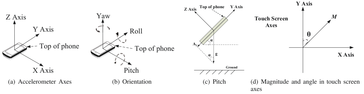
Fig. 2. Illustration of sensing values
