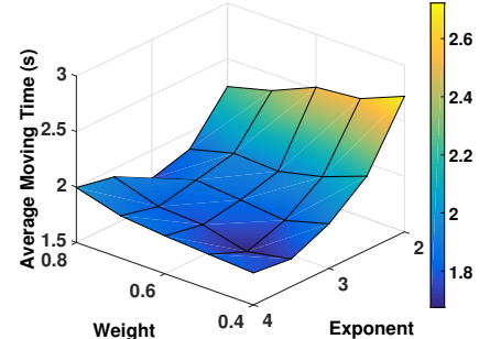
Fig. 10. Moving time versus weight and exponent with multiplier=6
