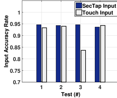
Fig. 15. Input accuracy rate using Android phones and a numeric keypad
