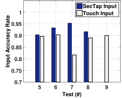
Fig. 16. Input accuracy rate using Android phones and a QWERTY keyboard
