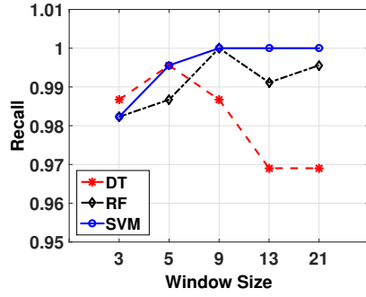
Fig. 5. Recall versus window size
