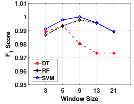
Fig. 7. F_1 score versus window size
