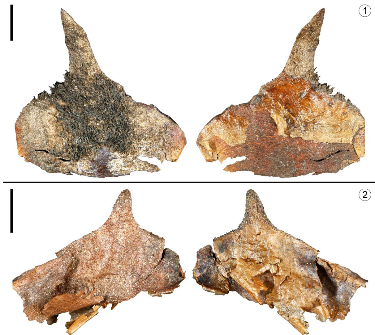
Plate 5. Early Cretaceous bract-scales of Cycadolepis sp. from Tevshiin Govi. Light micrographs. 1. Broadly ovate bract-scale with acuminate spine-like apex, showing adaxial (left) and abaxial surfaces (right). Note tightly intertwined, tomentose covering of trichomes on adaxial surface, while abaxial surface (right) has trichomes only near margin of scale (PP56994); 2. Broadly ovate bract-scale with acuminate apex with rounded tip, showing adaxial (left) and abaxial surfaces (right). Note tightly intertwined, tomentose covering of trichomes on adaxial surface (right), while abaxial surface has trichomes only near margin of scale (PP56995). Scale bars = 2 mm
