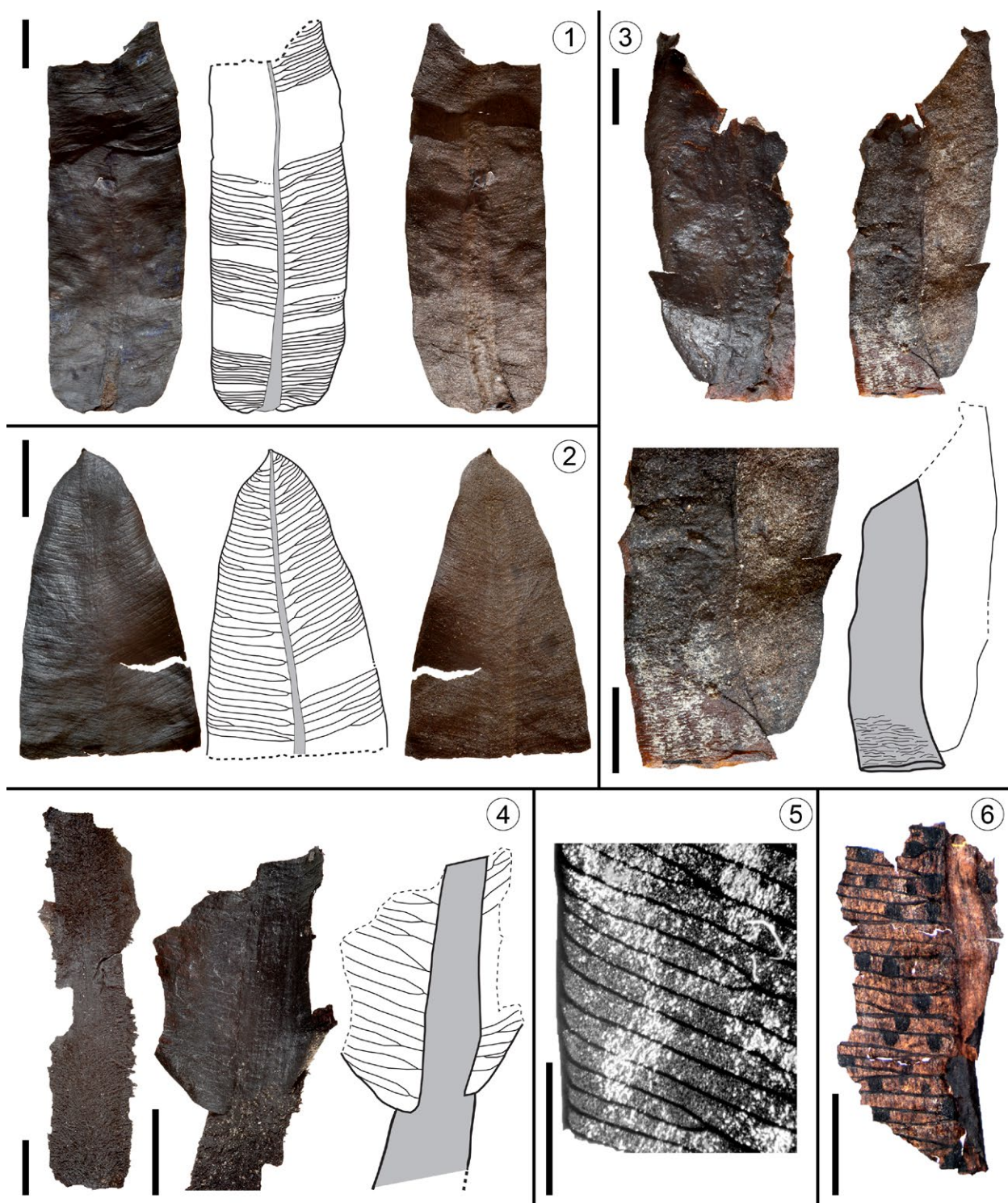
Plate 1. Early Cretaceous leaves of Nilssoniopteris tomentosa sp. nov. from Tevshiin Govi. Light micrographs and line drawings. 1. Holotype (PP56982), showing leaf base and midrib; leaf apex missing. Left, adaxial surface; center, line drawing of adaxial surface, showing stout midrib and dichotomizing lateral veins; right, abaxial surface, showing light brown/red-brownish color; 2. Leaf fragment, showing acute, slightly acuminate apex. Left, adaxial surface; center, line drawing of adaxial surface, showing stout midrib and dichotomizing lateral veins; right, abaxial surface, showing light brown/red-brownish color (PP56983); 3. Leaf fragment, showing basal part of lamina. Upper left, adaxial surface; upper right, abaxial surface, showing stout midrib with transverse striations; bottom left, detail of leaf base, showing broad, stout midrib; bottom right, line drawing from figure on upper right, showing stout midrib in grey (PP56984); 4. Leaf fragment, showing basal part of leaf lamina, midrib and petiole. Left, abaxial surface, showing petiole and midrib covered with tomentose trichomes; center, detail of leaf base from adaxial surface; right, line drawing of leaf base from adaxial surface, showing stout midrib/petiole (dark grey) and insertion of lamina into upper part of midrib (PP56985); 5. Portion of cleared leaf from near leaf margin, showing dichotomous and unbranched lateral veins that curve exmedially toward leaf apex (PP56986); 6. Fragment of adaxial leaf cuticle, showing leaf lamina with several lateral veins dichotomizing close to midrib. Dark spots represent wound tissue likely caused by insect galls (PP56987). All scale bars = 3 mm
