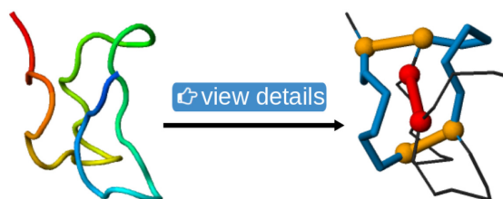
Figure 13. The result of the ‘View details’ button on the structure visualization. The loop-forming subchains are in blue, the loop-forming bridges are in orange, and the loop-piercing bridge is in red.
