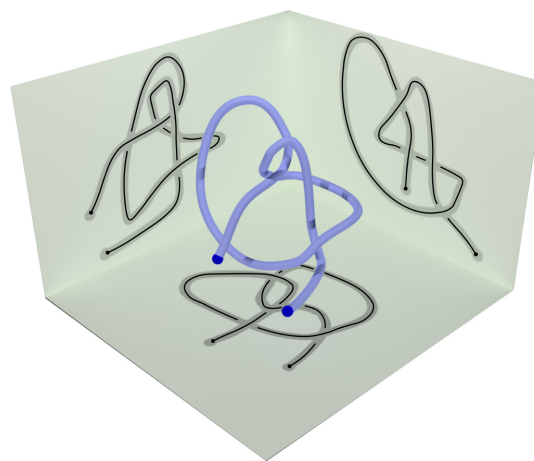
Figure 4. A knotoid is defined via a projection of an open 3D curve onto a plane. Its knotoid type depends on the choice of the plane.
