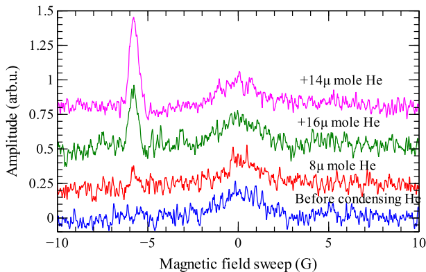
Fig. 6 ESR electron line evolution in “pure” Ne Sample 1 ( [H_2] = 100 ppm) during condensing He into the sample cell. The narrow line on the left is the e\text{-}H_2 line, which grows after condensing helium into the sample cell (Color figure online)
