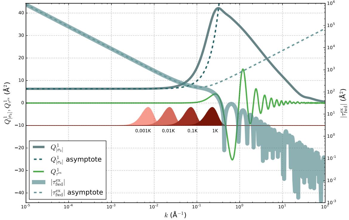
Figure B1. Accuracy of approximations at different momenta/temperatures. The figure shows Q_{[\sigma k]}^1 , \tau_{\text{fwd}}^{\text{ex}} for atomic hydrogen with their series expansions equations (8) and (9), as well as Q_{[\tau^{\text{ex}}]}^1 . These quantities are multiplied with a Gaussian and integrated over all momenta; a few Gaussians for a few different temperatures are shown. For high enough momenta the series expansions naturally break down, so in order for the asymptotic formula to give a good approximation to \mu the Gaussian should be concentrated in the area where the series expansions approximate the quantities well. This gives upper bounds T_Q and T_\tau on temperature where the asymptotic formula can be expected to work.
