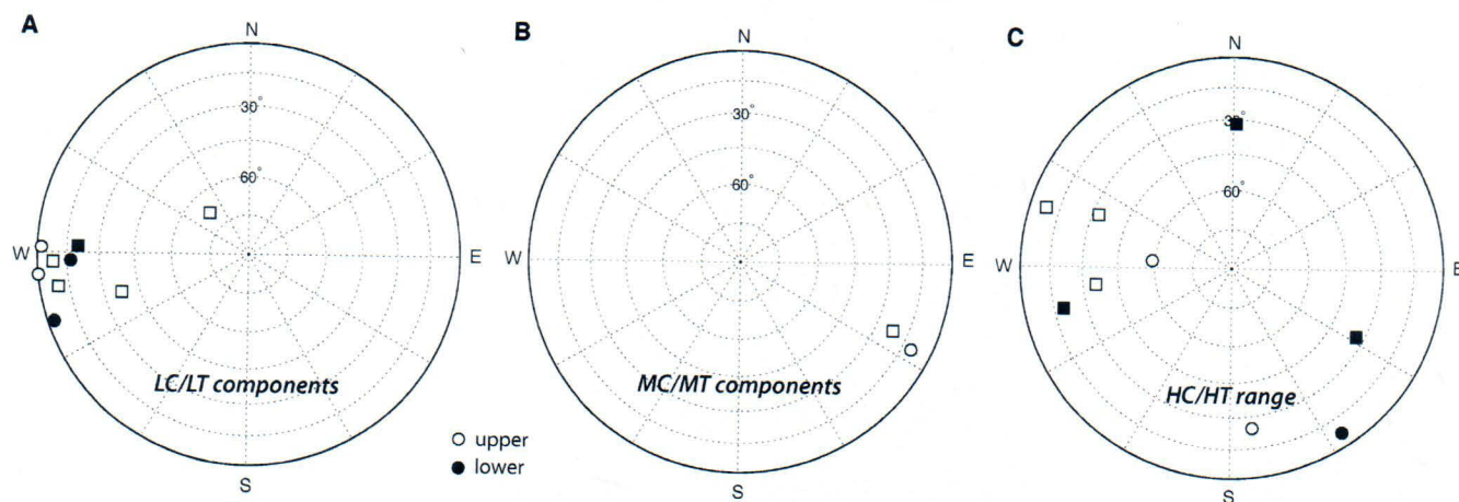
Fig. 7. NRM component directions observed in NWA 7325. Shown are equal area stereographic projections of Fisher mean directions (symbols) and associated maximum angular deviation values (surrounding ellipses) obtained from principal component analyses. (A) LC (circles) and LT (squares) component directions. (B) MC (circles) and MT (squares) magnetization directions. (C) HC (circles) and HT (squares) magnetization directions.
