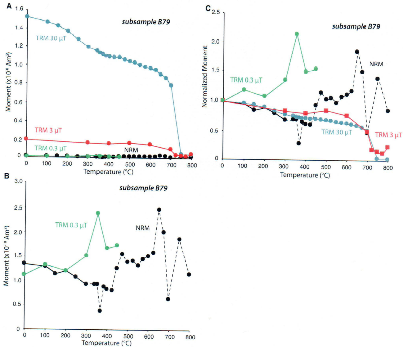
Fig. 10. Thermal demagnetization of NRM (black curve and points) compared to total TRM acquired from cooling in a field of 800 °C in fields of 30, 3, and 0.3 \mu\text{T} (blue, red, and green curves and points, respectively) for sample B79. (A) All data, expressed as moment as a function of temperature. (B) Zoom into NRM and 0.3 \mu\text{T} TRM data from (A). (C) Moment normalized to moment at room temperature before starting thermal demagnetization. NRM loses directional stability by a demagnetization temperature of 300 °C; directionally unstable data at higher demagnetization temperatures are connected with a dashed line. (For interpretation of the references to color in this figure legend, the reader is referred to the web version of this article.)
