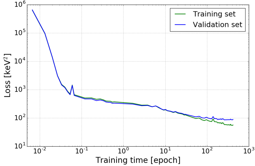
Figure 5. The learning curve shows the decreasing loss during training of the DNN. Thus, the DNN is learning to predict the energy from a waveform.
