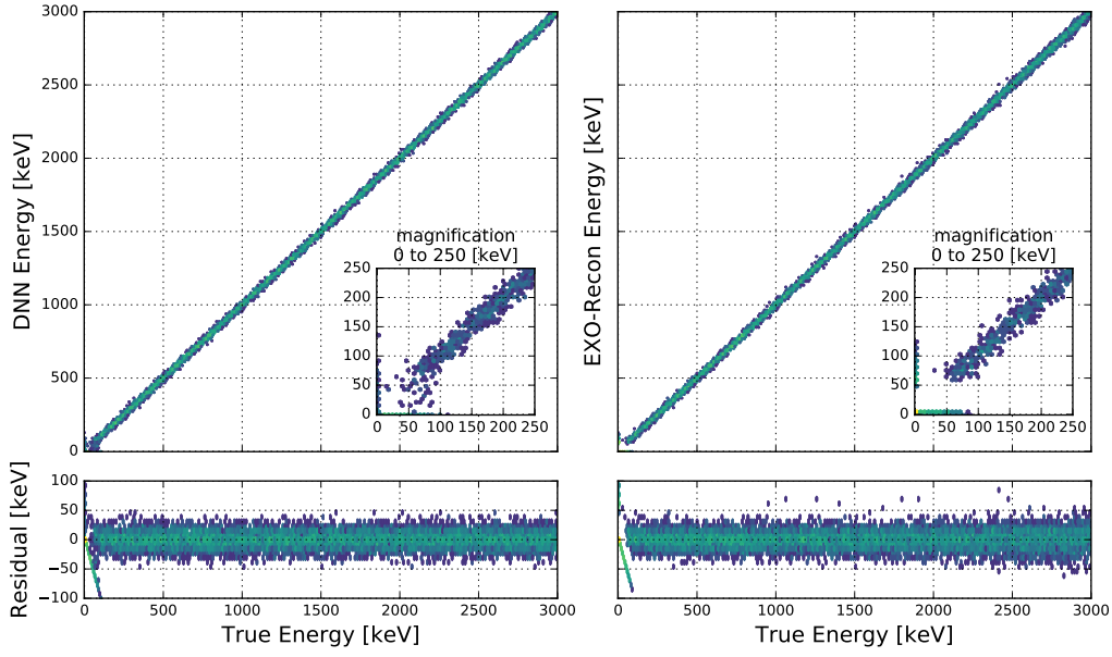
Figure 6. Predicted/reconstructed energy for the test set with both methods, DNN and EXO-recon.
