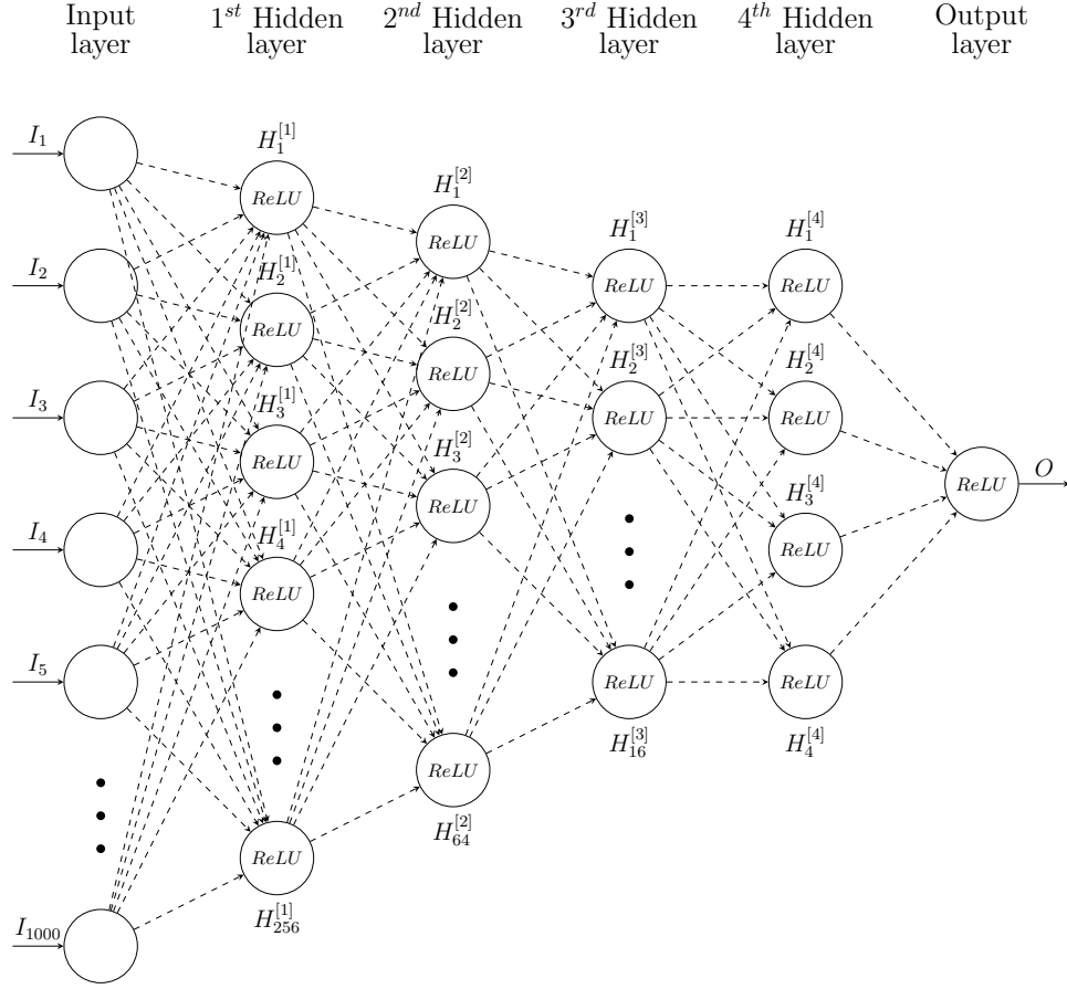
Figure 4. The architecture of the DNN used for the U-Wire study. The input layer represents the input waveform with 1000 data points. It is fed to the first hidden layer, which has 256 neurons with rectified linear unit (ReLU) activation functions. The number of neurons per layer is gradually decreased from 256 to 64, then to 16, then to 4, and then to 1 in the output layer. The DNN is trained to output the true energy in the output layer. The model contains 273 817 trainable parameters.
