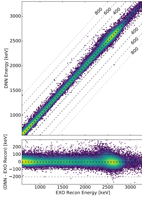
Figure 16. Energies of experimental events from a ^{228}\text{Th} calibration source at position S5 reconstructed by the neural network as function of the energy reconstructed by the conventional analysis. The corresponding residuals are shown in the lower panel. The color denotes the intensity on a logarithmic scale. Dashed lines indicate a certain residual as given in the figure. The residual of both methods does not show systematic energy dependent features.
