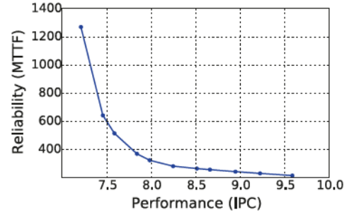
Figure 1: Reliability vs. Performance for HMA averaged over astar, cactusADM, mix1 benchmarks (methodology in Section 4) running on a 16 core multicore. Individual points reflect different proportions of hot pages placed in the faster stacked RAM.
