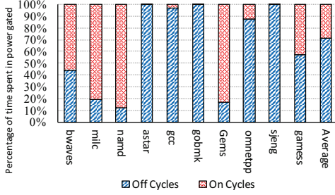
Figure 15: Percentage of time that CSD power gates VPU.
