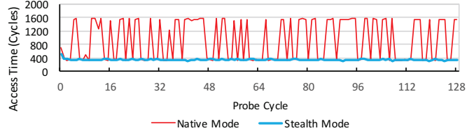
(b) FLUSH+RELOAD on RSA
