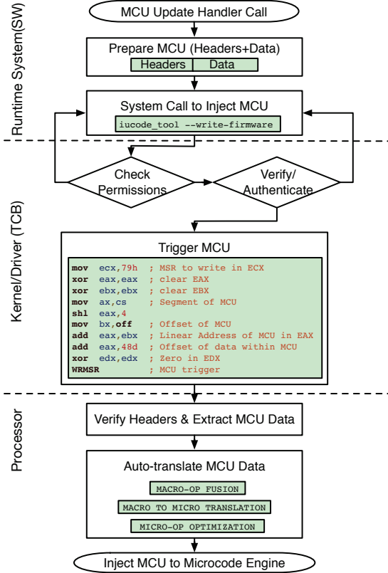
Figure 2: Auto-translation Procedure
