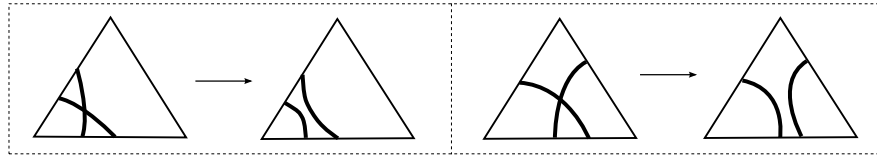
Figure 18. There are two types of double points (up to isotopies and rotations); in each case the only resolution without returning arc is drawn. Other resolutions have returning arcs
