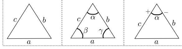
Figure 11. Ideal triangle \mathfrak{T} (left), with arcs \alpha, \beta, \gamma (middle), and \alpha(+ -) (right).
