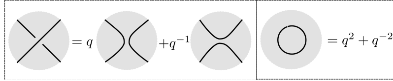
Figure 1. Skein relation (left) and trivial loop relation
