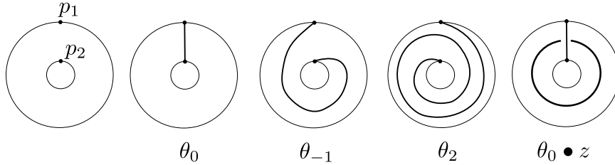
Figure 3. Marked annulus \mathbb{A}_{io} , arcs \theta_0, \theta_{-1}, \theta_2 , and element \theta_0 \bullet z
