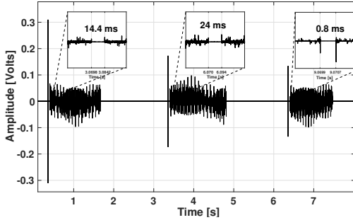
(b) Recorded output signal (in electrical domain) of the SEANet IoUT.
