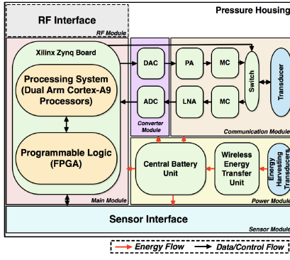
(a) SEANet IoUT hardware architecture.
