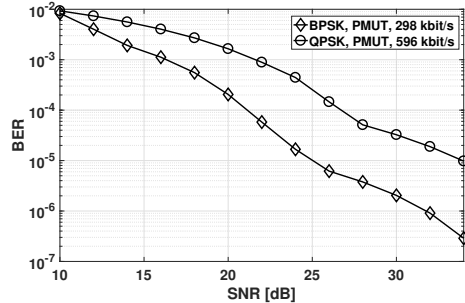
(c) BER versus SNR for different modulation schemes (BPSK and QPSK)
