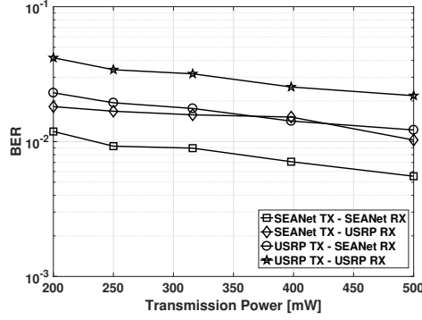
(a) BER versus transmission power for different pairs of platform.
