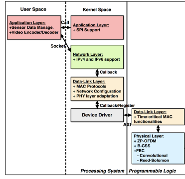
(b) SEANet IoUT software architecture.
