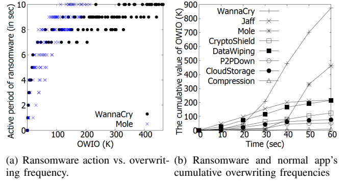
Fig. 1: Ransomware’s overwriting behavior (WannaCry, Jaff, Mole, and CryptoShield ransomwares): (a) There is a strong correlation between active period of ransomware and the number of overwrites per second ( = OWIO ), and (b) Cumulative values of overwrites show that ransomware does overwriting very frequently.
