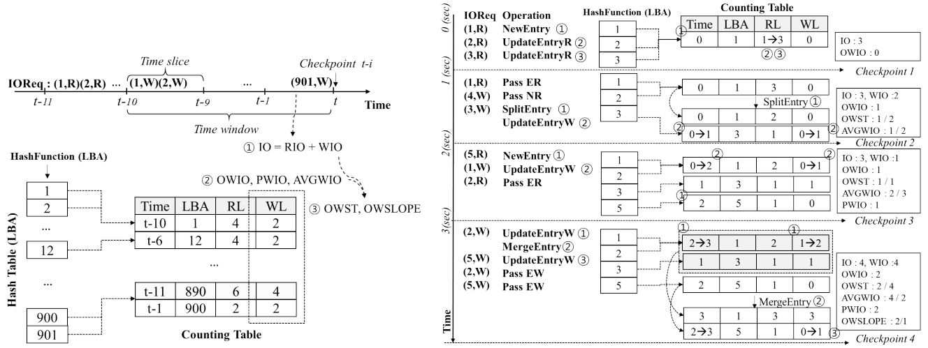
(a) Counting table holds the run-length of overwritings for each time slice. (b) Counting table update example using basic functions (NewEntry, UpdateEntryR, SplitEntry, UpdateEntryW, and MergeEntry)
