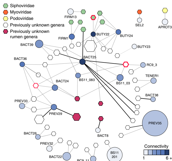
Fig. 6 | Host-viral interaction network. Viral genomes (hexagons) are connected to predicted microbial host genomes (circles) by edges. All genomes (viral and microbial) are sized by abundance across data sets. Viral genomes or contigs are coloured by taxonomic assignment. Microbial host MAGs are coloured by connectivity noted on the bottom right. An edge was drawn if a confident link could be established by tetranucleotide frequency (grey edges) or protospacers within the CRISPR-Cas-associated protein (Cas) systems (black edges). The length of the edge has no meaning. Viral genomes or contigs with proteins detected in proteomics are outlined in red.
