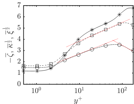
FIGURE 8. Mean scalar measures, plotted in equivalent dimensions, as functions of y^+ . The solid line with star symbols ( \text{---}\star\text{---} ) is minus the mean volume ratio: -\bar{\zeta} = -\langle\zeta\rangle , the dashed line with square symbols ( \text{---}\square\text{---} ) is the square-root of the mean geodesic distance from the identity: \bar{\kappa}^{\frac{1}{2}} = \sqrt{\langle\kappa\rangle} , the dashed-dot line with circle symbols ( \text{---}\circ\text{---} ) is the square-root of the mean anisotropy index: \bar{\xi}^{\frac{1}{2}} = \sqrt{\langle\xi\rangle} . Red dotted lines ( \text{---}\cdot\text{---} ) are logarithmic fits to the profiles: the fit to the \bar{\kappa}^{\frac{1}{2}} profile ( \text{---}\square\text{---} ) is given by 0.725 \log y^+ + 2.15 , the fits to the \bar{\xi}^{\frac{1}{2}} profile ( \text{---}\circ\text{---} ) are given by 0.65 \log y^+ + 1.20 and -0.9 \log y^+ + 7.6 . Note that the symbols are identifiers and are thus only a small subset of all the data points used in the line plots.
