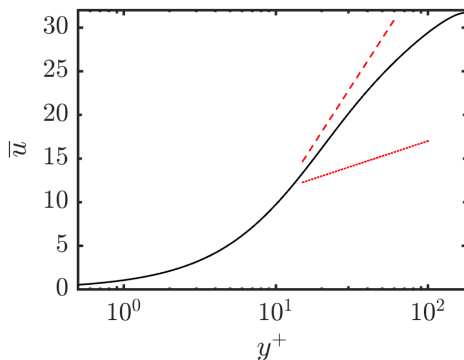
FIGURE 2. Mean velocity profile from a FENE-P drag-reduced channel flow simulation. The solid line (—) is the mean streamwise velocity, the red dotted (lower) line (---) is the von Kármán log-law, \bar{u}_{\text{von Kármán}}^+ = 2.5y^+ + 5.5 , and the red dashed (upper) line (---) is Virk's asymptote, \bar{u}_{\text{Virk}}^+ = 11.7y^+ - 17.0 .
