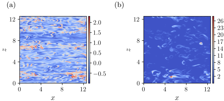
FIGURE 7. Wall-parallel (x, z) planes of isocontours of instantaneous C'_{xx}/\overline{C}_{xx} at (a) y^+ = 15 (b) y^+ = 180 (centreline), where \overline{C}_{xx}(y^+ = 15) = 2.22 \times 10^3 and \overline{C}_{xx}(y^+ = 180) = 1.02 \times 10^2 . The limits of the divergent colour map are set at the planar maxima and minima of C'_{xx}/\overline{C}_{xx} .
