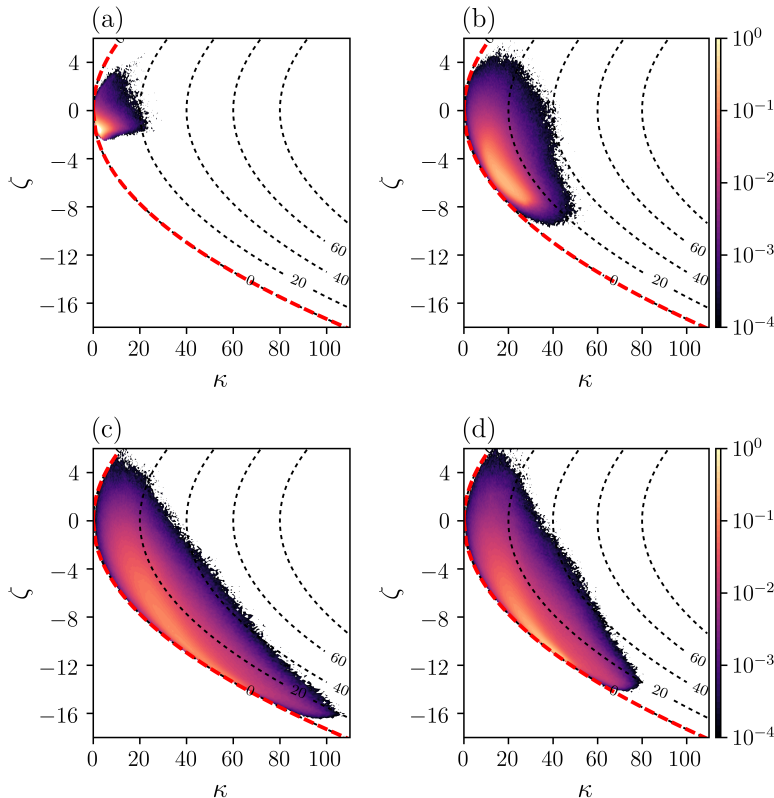
FIGURE 9. Joint probability density functions (JPDF) of the logarithmic volume ratio, \zeta , and the geodesic distance from the identity, \kappa , at four different wall-normal locations: (a) y^+ = 2 , (b) y^+ = 15 , (c) y^+ = 100 and (d) y^+ = 180 (centreline). Dotted lines (-----) are isocontours of the anisotropy index, \xi . The thick red dashed line (---) denotes the realizability bound, \kappa = \frac{1}{3}\zeta^2 , derived in (4.18), which coincides with the zero anisotropy index isocontour ( \xi = 0 ).
