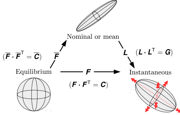
FIGURE 1. Schematic of the decomposition given in (3.5) and (3.6). The tensor \mathbf{F} is a composition of \bar{\mathbf{F}} and \mathbf{L} .
