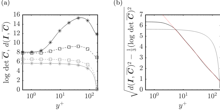
FIGURE 4. Scalar measures applied to nominal conformation tensors, in equivalent dimensions, plotted as functions of y^+ . (a) The solid line with star symbols ( \text{---}\star\text{---} ) is \log \det \bar{\mathbf{C}} , the logarithmic volume; the dashed line with square symbols ( \text{---}\square\text{---} ) is d(\mathbf{I}, \bar{\mathbf{C}}) , the geodesic distance between \bar{\mathbf{C}} and \mathbf{I} on \text{Pos}_3 , (b) anisotropy index, \sqrt{d(\mathbf{I}, \bar{\mathbf{C}})^2 - \frac{1}{3}(\log \det \bar{\mathbf{C}})^2} , which is the geodesic distance from the closest isotropic tensor. For both (a) and (b), black lines are for \bar{\mathbf{C}} = \langle \mathbf{C} \rangle and grey lines are when \bar{\mathbf{C}} is equal to the FENE-P laminar conformation tensor. The red dotted line ( \text{---}\cdot\text{---} ) in (b) is -1.375 \log y^+ + 7.925 . Note that the symbols in (a) are identifiers and are thus only a small subset of all the data points used in the line plots.
