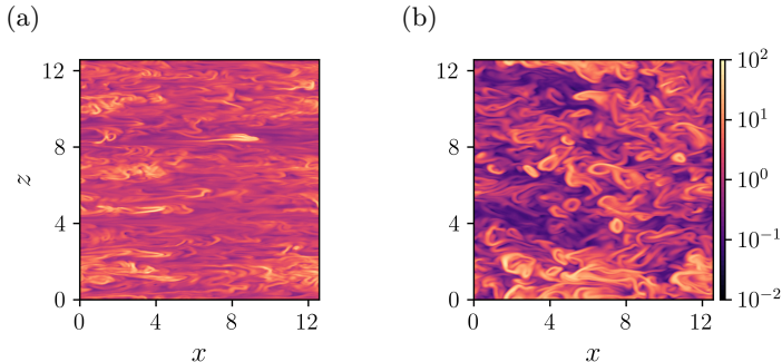
FIGURE 5. Wall-parallel (x, z) planes of isocontours of instantaneous I_{\mathbf{G}} = \text{tr } \mathbf{G} . (a) at y^+ = 15 and (b) y^+ = 180 (centreline).
