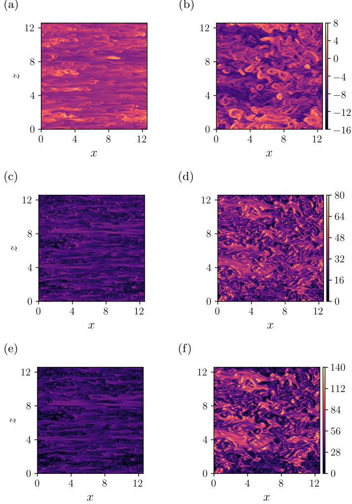
FIGURE 6. Wall-parallel (x, z) planes of isocontours of instantaneous (a)–(b): logarithmic volume ratio, \zeta , (c)–(d): geodesic distance from the identity, \kappa , and (e)–(f): anisotropy index, \xi . (a), (c), and (e): y^+ = 15 . (b), (d), and (f): y^+ = 180 (centreline).
