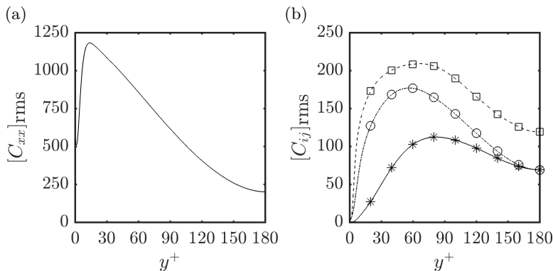
FIGURE 10. Root-mean-square profiles of \mathbf{C}' , [C_{ij}]_{\text{rms}} = \sqrt{\langle C_{ij}^2 \rangle - \langle C_{ij} \rangle^2} based on the Reynolds decomposition (1.1). (a) [C_{xx}]_{\text{rms}} (b) the solid line with star symbols ( -\ast- ) is [C_{yy}]_{\text{rms}} , the dashed line with square symbols ( --\square-- ) is [C_{zz}]_{\text{rms}} , and the dashed-dot line with circle symbols ( -\circ- ) is [C_{xy}]_{\text{rms}} . Note that the symbols in (b) are identifiers and are thus only a small subset of all the data points used in the line plots.
