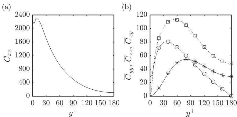
FIGURE 3. Mean conformation tensor profiles from a FENE-P drag-reduced channel flow simulation. (a) \bar{C}_{xx} (b) the solid line with star symbols (—*—) is \bar{C}_{yy} , the dashed line with square symbols (---□---) is \bar{C}_{zz} , and the dashed-dot line with circle symbols (---○---) is \bar{C}_{xy} . The remaining components of the mean conformation tensor are 0. Note that the symbols in (b) are identifiers and are thus only a small subset of all the data points used in the line plots.
