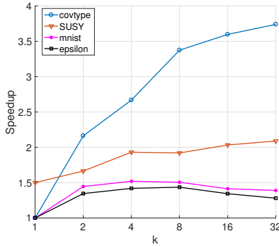
Figure 7: Speedup results for PN method with RC-SFISTA as inner solver compared to FISTA used as inner solver.
