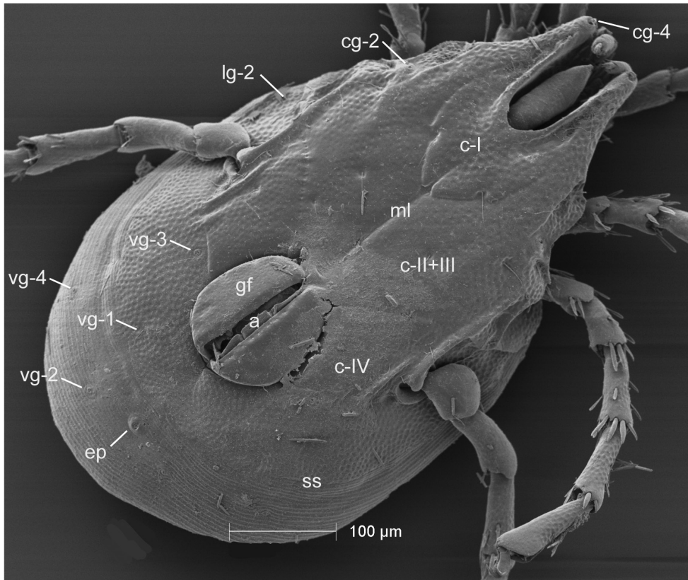
Figure 4. Testudacarine male venter (SEM): coxo-glandularia (cg); latero-glandularia (lg); ventro-glandularia (vg); coxae (c); coxae-II+III midline (ml); genital field (gf); acetabula (a); line of secondary sclerotization (ss); excretory pore (ep). Scale: 100 \mu m. Photo Michelle Hoppner and Ian Smith (used with permission).
