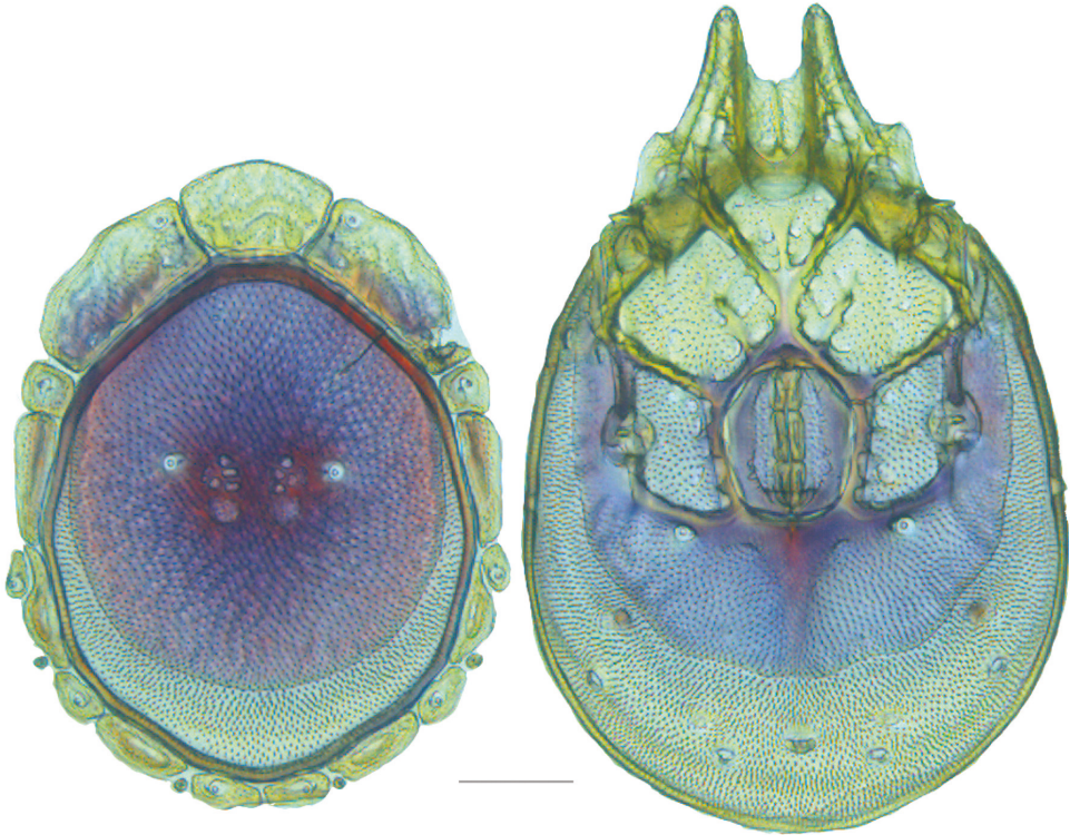
Figure 26. Testudacarus harrisi female: (Left) dorsum; (Right) venter. Scale: 100 \mu m.
