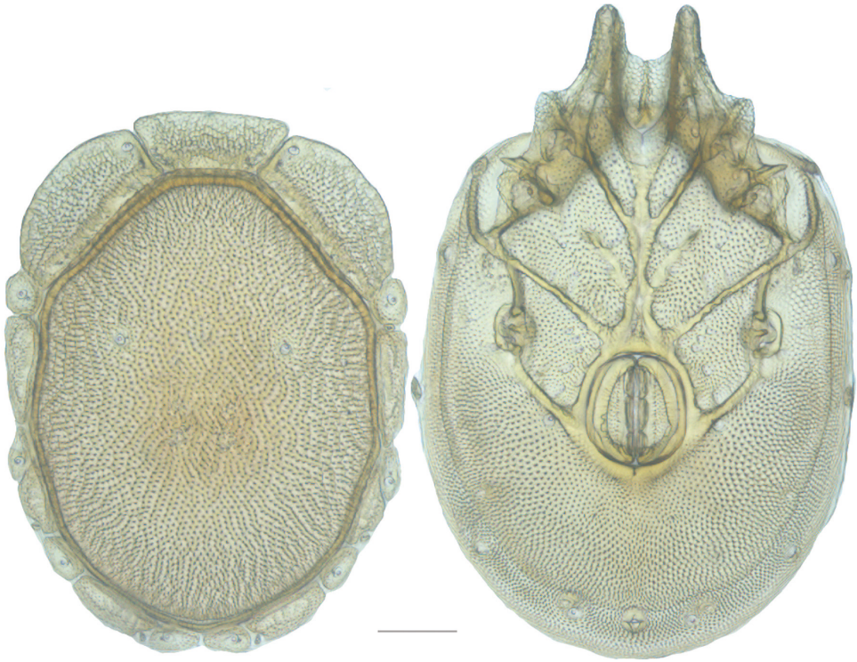
Figure 34. Testudacarus americanus male: (Left) dorsum; (Right) venter. Scale: 100 \mu m.
