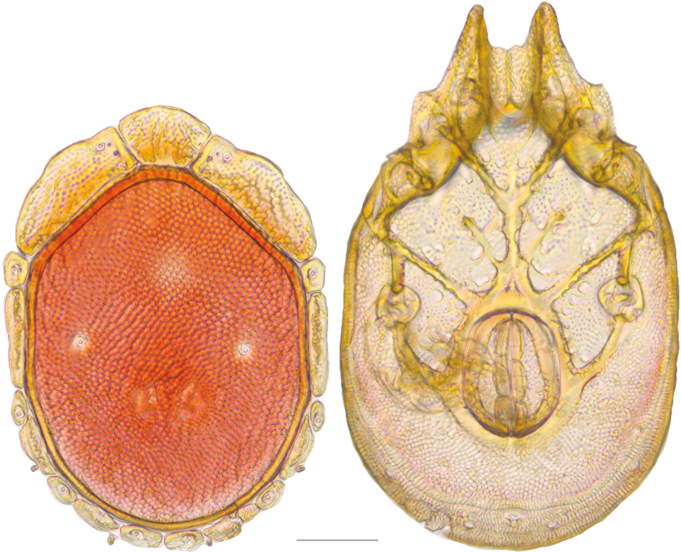
Figure 15. Testudacarus minimus male: (Left) dorsum; (Right) venter. Scale: 100 \mu m.
