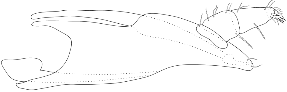
Figure 9. Debsacarus oribatoides gnathosoma (generalized).
