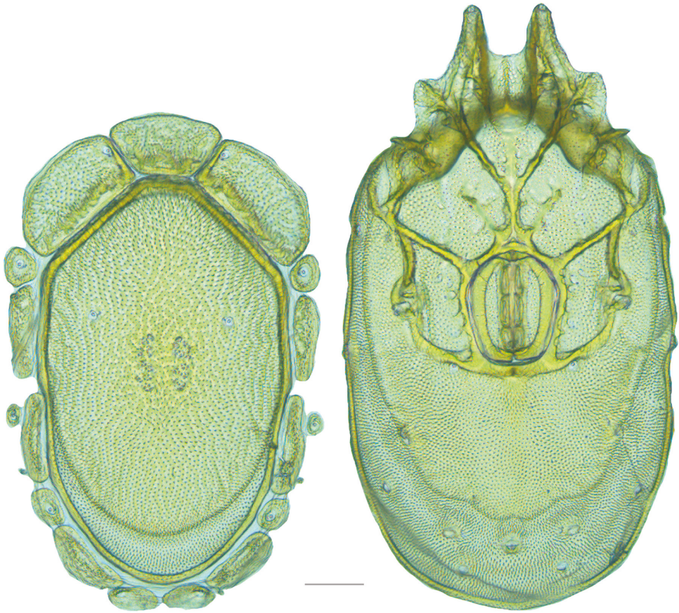
Figure 47. Testudacarus oblongatus female: (Left) dorsum; (Right) venter. Scale: 100 \mu m.
