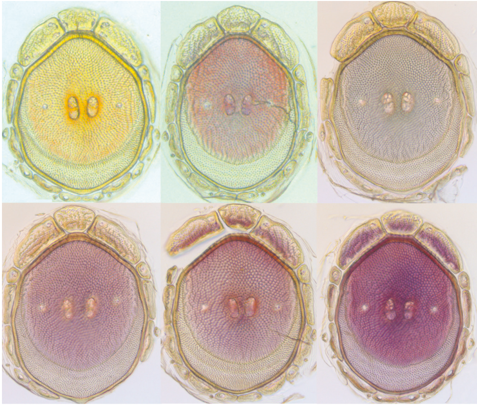
Figure 17. Testudacarus vulgaris color variation.
