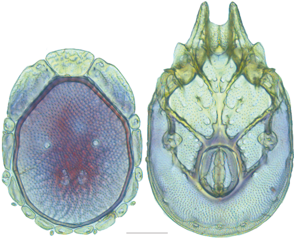
Figure 27. Testudacarus harrisi male: (Left) dorsum; (Right) venter. Scale: 100 \mu m.
