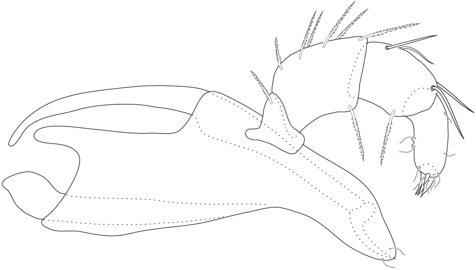
Figure 36. Testudacarus hyporhynchus sp. n. gnathosoma (generalized).
