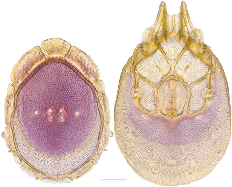
Figure 16. Testudacarus vulgaris female: (Left) dorsum; (Right) venter. Scale: 100 \mu m.
