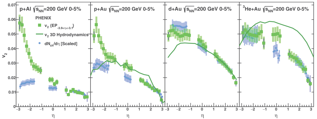
FIG. 4. Elliptic flow v_2 as a function of pseudorapidity in high-multiplicity 0%–5% central p + \text{Al} , p + \text{Au} , d + \text{Au} , and ^3\text{He} + \text{Au} collisions at \sqrt{s_{NN}} = 200 GeV. Also shown are predictions from the hydrodynamical model [4]. Lastly, the measured dN_{\text{ch}}/d\eta results are shown scaled to match the v_2 at forward rapidity for shape comparison with the elliptic flow coefficients.
