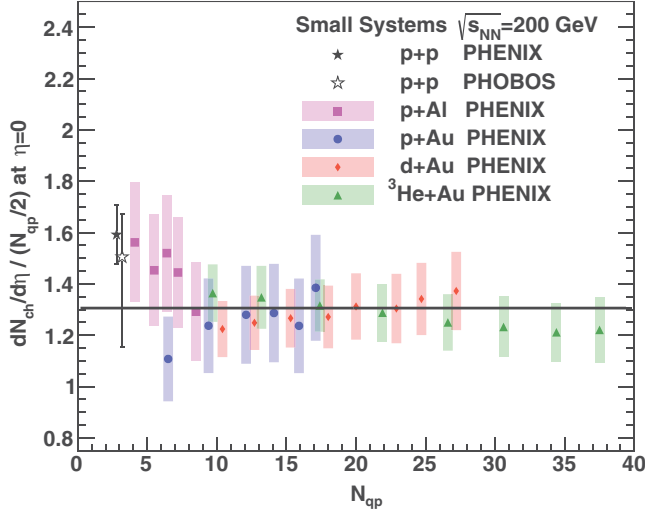
FIG. 3. Midrapidity charged hadron dN_{\text{ch}}/d\eta per participating quark pair ( N_{qp}/2 ) as a function of the number of participating quarks ( N_{qp} ). Results are shown for p + \text{Al} , p + \text{Au} , d + \text{Au} , and ^3\text{He} + \text{Au} collisions in various multiplicity classes. Also shown are previously published results in p + p collisions from PHENIX [15] and PHOBOS [27]. The line is the best fit to all the data to a constant level.
