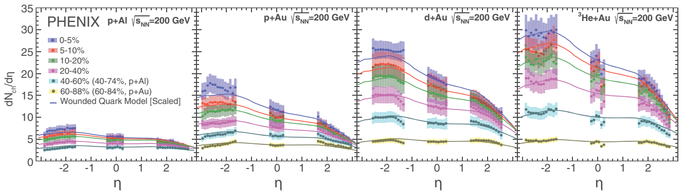
FIG. 2. Charged hadron dN_{\text{ch}}/d\eta as a function of pseudorapidity in various multiplicity classes of p + \text{Al} , p + \text{Au} , d + \text{Au} , and ^3\text{He} + \text{Au} collisions at \sqrt{s_{\text{NN}}} = 200 GeV. Predictions from the wounded-quark model [3] are shown.
