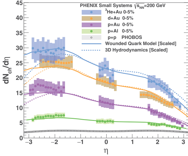
FIG. 1. Charged hadron dN_{\text{ch}}/d\eta as a function of pseudorapidity in high-multiplicity 0%–5% central ^3\text{He} + \text{Au} , d + \text{Au} , p + \text{Au} , and p + \text{Al} collisions at \sqrt{s_{\text{NN}}} = 200 GeV. Also shown are results in inelastic p + p collisions at \sqrt{s_{\text{NN}}} = 200 GeV as measured by the PHOBOS Collaboration [27]. Predictions from the wounded-quark [3] and hydrodynamical [4] models are shown. The calculations have an overall normalization factor ( S ) to best match the data. These factors are S = 0.88, 0.93, 0.85 , and 0.77 for the wounded-quark model for p + \text{Al} , p + \text{Au} , d + \text{Au} , and ^3\text{He} + \text{Au} , respectively; and S = 0.81, 0.96 , and 0.75 for the hydrodynamical model for p + \text{Au} , d + \text{Au} , and ^3\text{He} + \text{Au} , respectively.
