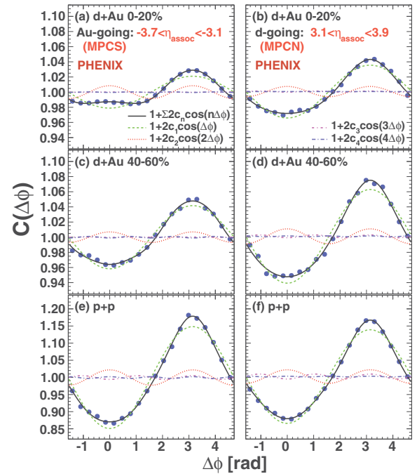
FIG. 5. Centrality dependence of correlation functions for d + \text{Au} and p + p collisions at \sqrt{s_{NN}} = 200 GeV for \pi^0 in |\eta_{\text{trig}}| < 0.35 (CNT). (a), (c), (e) \pi^0 are associated with the towers in MPCS (Au-going direction) and (b), (d), (f) MPCN ( d -going direction), for 3 < p_T < 3.5 GeV/c.
