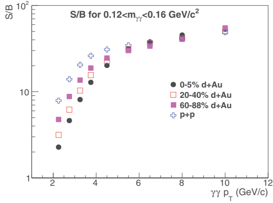
FIG. 3. Centrality and \gamma\gamma p_T dependence of the signal to combinatoric background ratio ( S/B ) for pairs in the 0.12 < m_{\gamma\gamma} < 0.16 GeV/ c^2 mass window.
