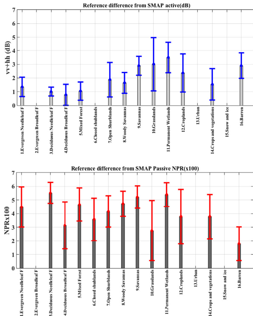
Fig. 4. (Top) SMAP reference differences for the active (dB) and (bottom) passive (NPR) cases over 13 land cover classes north of 45°. Coloured vertical lines indicate \pm 1 standard deviation.
