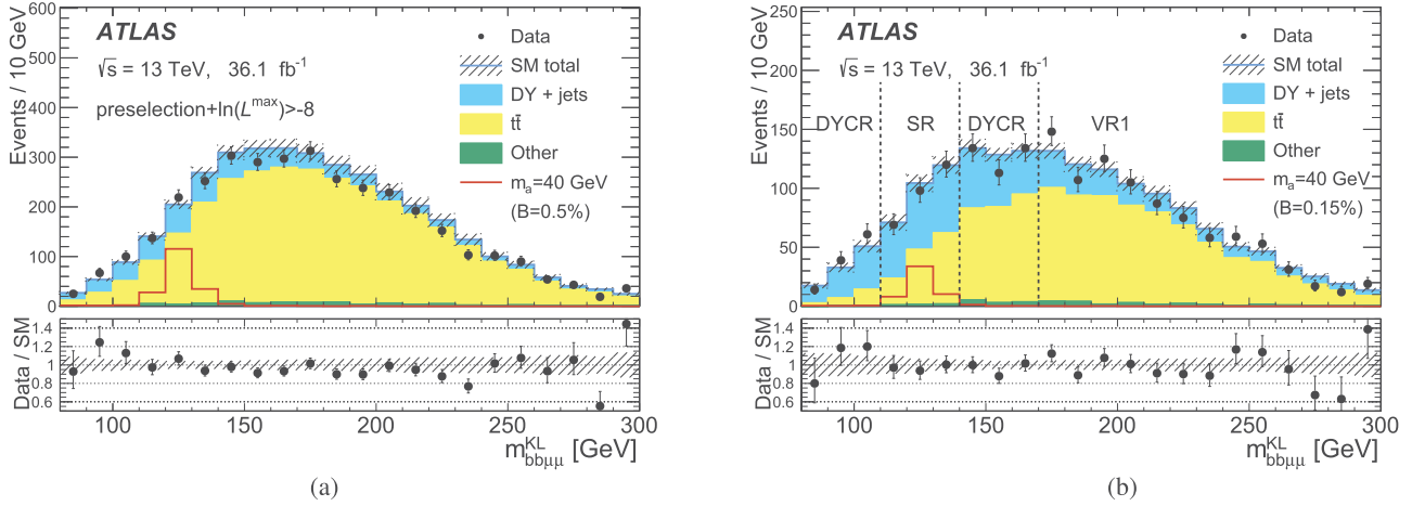
Fig. 3. The predicted and observed m_{bb\mu\mu}^{KL} distributions (a) after the preselection and the KL-fit \ln(L^{\max}) > -8 constraint and (b) across DYCR, SR and VR1 (shown separated by vertical dashed lines). Both are shown after the background-only fit and differ only in the E_T^{\text{miss}} < 60 GeV criterion being applied in (b). The signal distribution for m_a = 40 GeV is also shown assuming the SM Higgs boson cross-section (including ggF, VBF and VH production) and (a) \mathcal{B}(H \rightarrow aa \rightarrow bb\mu\mu) = 0.5\% and (b) \mathcal{B}(H \rightarrow aa \rightarrow bb\mu\mu) = 0.15\% . The hashed bands show the total statistical and systematic uncertainties of the backgrounds.
