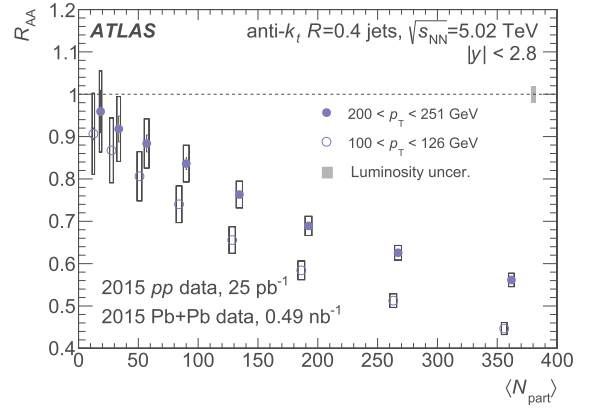
Fig. 6. The R_{AA} values for jets with 100 < p_T < 126 GeV and 200 < p_T < 251 GeV for rapidity |y| < 2.8 evaluated as a function of \langle N_{part} \rangle . For legibility, the \langle N_{part} \rangle values are shifted by -7 and +7 for 100 < p_T < 126 GeV selection and 200 < p_T < 251 GeV selection, respectively. The error bars represent statistical uncertainties. The heights of the open boxes represent systematic uncertainties. The widths of the open boxes represent the uncertainties in the determination of \langle N_{part} \rangle . The grey shaded box at unity represents the uncertainty of the Pb+Pb integrated luminosity.
