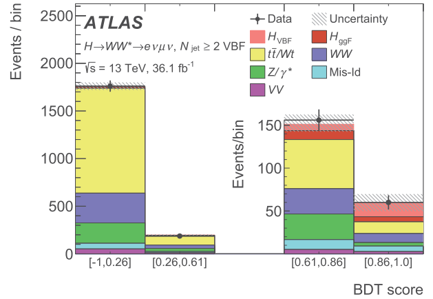
Fig. 5. Post-fit BDT score distribution with the signal and the background modelled contributions in the VBF signal region. The hatched band shows the total uncertainty of the signal and background modelled contributions.
