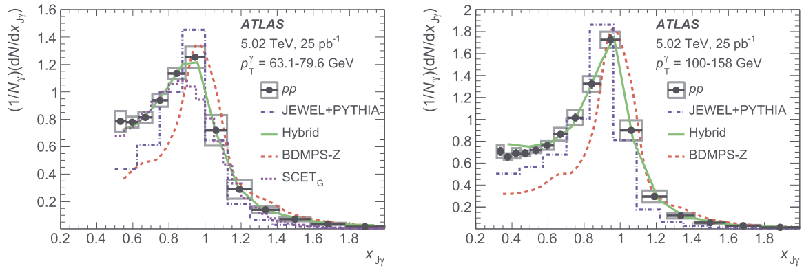
Fig. 9. Photon-jet p_T -balance distributions (1/N_\gamma)(dN/dx_{j\gamma}) in pp collisions for (left) p_T^\gamma = 63.1-79.6 GeV and (right) p_T^\gamma = 100-158 GeV. The unfolded results are compared with the theoretical calculations shown as dashed coloured lines (see text). Total systematic uncertainties are shown as boxes, while statistical uncertainties are shown as vertical bars.
