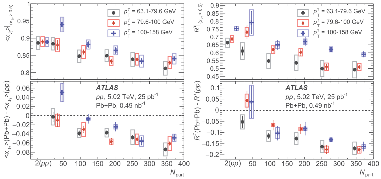
Fig. 8. Summary of (left) the mean jet-to-photon p_T ratio \langle x_{j\gamma} \rangle and (right) the total per-photon jet yield R^\gamma , calculated in the region x_{j\gamma} > 0.5 . The values are presented as a function of the mean number of participating nucleons N_{part} in top panels. Each colour and symbol represents a different p_T^\gamma interval, where the lowest and highest intervals are displaced horizontally for clarity. The points plotted at N_{part} = 2 correspond to pp collisions. The bottom panels show the difference between the Pb + Pb centrality selection and pp collisions. Boxes show the total systematic uncertainty while the vertical bars represent statistical uncertainties.
