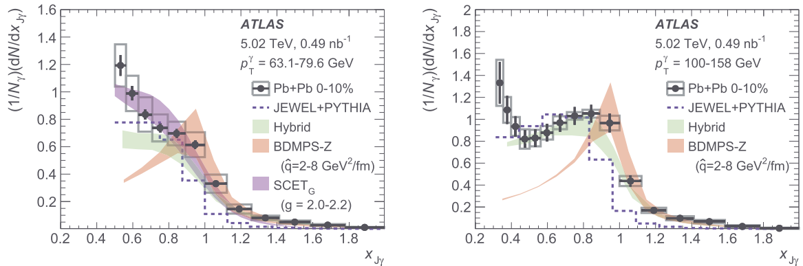
Fig. 10. Photon-jet p_T -balance distributions (1/N_\gamma)(dN/dx_{j\gamma}) in 0–10% Pb + Pb collisions for (left) p_T^\gamma = 63.1-79.6 GeV and (right) p_T^\gamma = 100-158 GeV. The unfolded results are compared with the theoretical calculations shown as dashed coloured lines denoting central values or coloured bands which correspond to a range of theoretical parameters (see text). Total systematic uncertainties are shown as boxes, while statistical uncertainties are shown as vertical bars.
