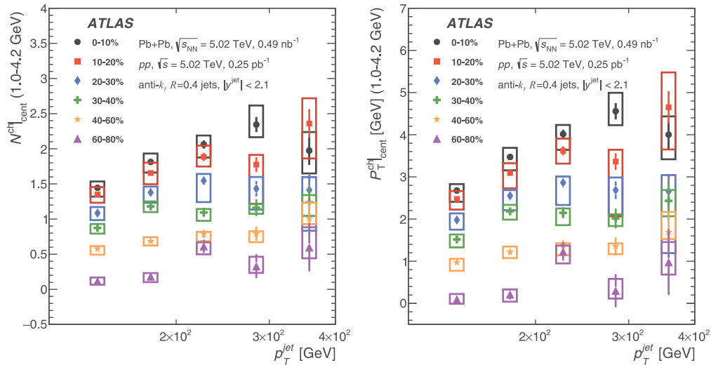
FIG. 23. Difference between Pb + Pb collisions and pp collisions in the total yield of charged particles N_{\text{cent}}^{\text{ch}} (left), and difference in the total transverse momentum carried by charged particles P_{\text{cent}}^{\text{ch}} (right) for particles with p_T from 1 < p_T < 4.2 GeV evaluated as a function of p_T^{\text{jet}} for six centrality intervals. The vertical bars on the data points indicate statistical uncertainties while the boxes indicate systematic uncertainties.
