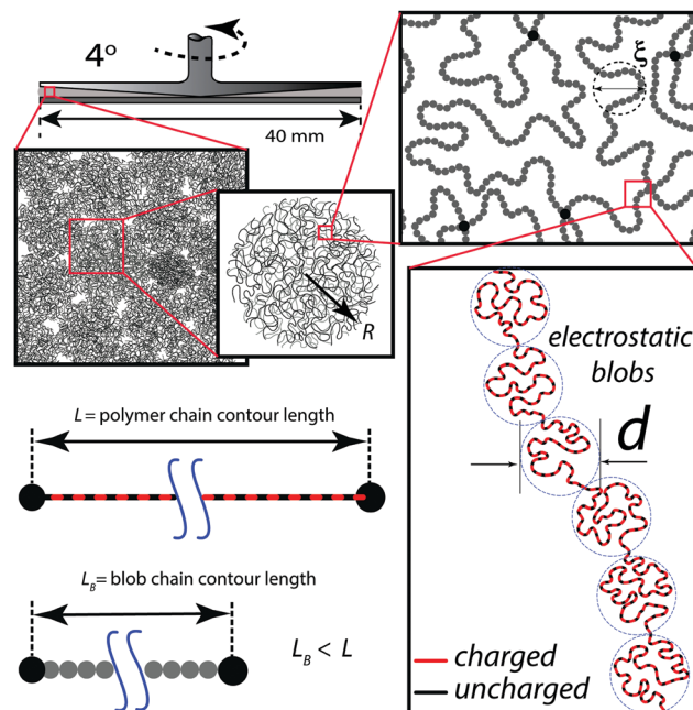
Fig. 1 Illustration of polyelectrolyte microgel hierarchical structure. Polyelectrolyte microgels swell and jam together to form a material that transitions between solid-like to fluid-like behaviors under applied shear stress. In contrast to neutral polymers, the polyelectrolyte backbone exhibits a hierarchical structure that comprises small electrostatic blobs of diameter d which arrange into larger fluctuating chains. The correlation length associated with these chains of blobs is the mesh size, \xi . This re-structuring of the polyelectrolyte backbone effectively reduces the polymer contour length L to a shorter blob chain contour length, L_B .
