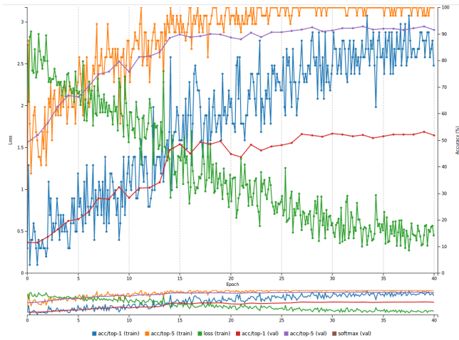
Figure 6: Accuracy graph over training iterations for ResNet18.
