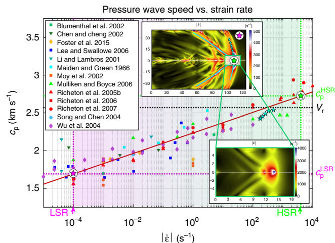
Fig. 3 Strain-rate dependence of the pressure wave speed in PMMA. The values of the pressure wave speeds c_p , computed based on the elastic moduli versus strain-rate data acquired from the literature as reported in the legend 32,34–37,48–55 , where the diamond symbols indicate tensile tests, as opposed to the other symbols that indicate compressive tests. The red solid line is a logarithmic fit of this data (see Methods section). The values of c_p for several locations along the pressure shock front (cyan stars), predicted from the relation (Eq. 1) between the inclination angles of the pressure shock front and rupture speed, are plotted vs. the strain rate determined at those locations. The two sets of pressure wave speeds (from the literature and from our experiments) show an excellent agreement, demonstrating that the inclination angles of the pressure shock fronts are consistent with the viscoelastic stiffening induced. The rupture speed V_r = 2.57 \text{ km s}^{-1} (dotted black line) is higher than all of those shock-wave determined pressure wave speeds, indicating that the rupture is supersonic with respect to them. The high-strain-rate (HSR) pressure wave speed, corresponding to the strain rate of about 4 \times 10^3 \text{ s}^{-1} at the crack tip (the blue region in the bottom inset), is determined as the wave speed on the logarithmic fit (red line) that corresponds to that strain rate (green star). The strain-rate level at the crack tip is obtained from a similar test performed on a sample at an angle \alpha = 29^\circ (rather than 30^\circ ) under the same loading conditions, by focusing on a smaller field of view, which enables a higher strain-rate resolution (lower inset). The low-strain-rate (LSR) pressure wave speed (see Discussion section) corresponds to the pressure wave speeds indicated by the horizontal green and purple dashed lines
