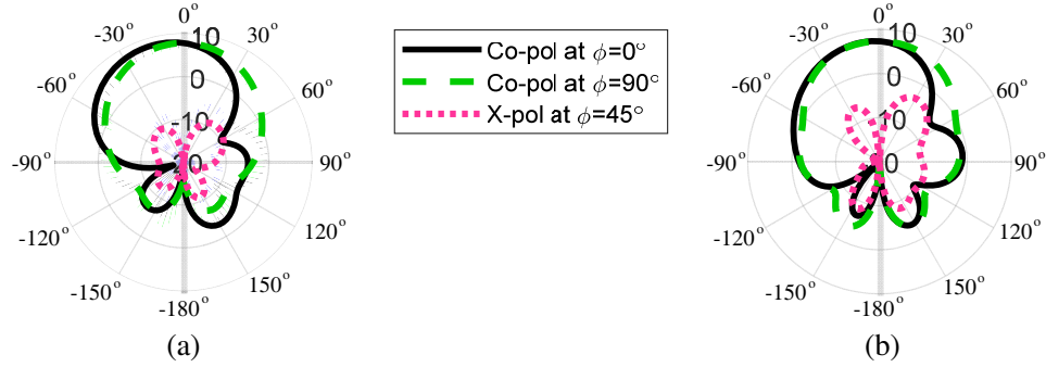
Figure 5. Co-polar radiation patterns at the principal planes and cross-pol radiation pattern at \phi = 45^\circ of the conformal U-slot patch antenna at (a) 9.5 GHz and (b) 11.5 GHz.
