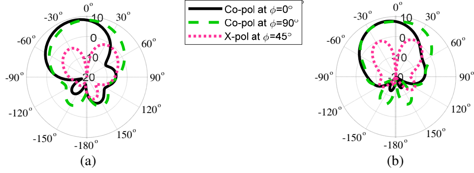
Figure 4. Co-polar radiation patterns at the principal planes and cross-pol radiation pattern at the \phi = 45^\circ of planar U-slot patch antenna at (a) 9.5 GHz and (b) 11.5 GHz.
