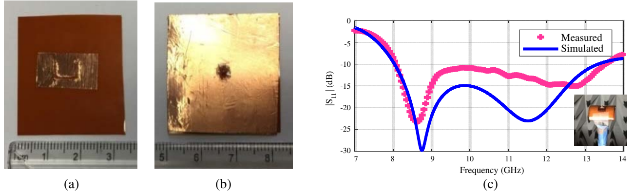
Figure 6. (a) Top and (b) bottom of the fabricated U-slot antenna made from adhesive copper tape placed on 150FN019 Kapton film and (c) simulated and measured S_{11} of the conformal U-slot antenna with \varepsilon_r = 1 , r = 15 mm, and \alpha = 100^\circ .
