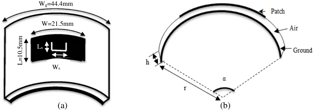
Figure 1. (a) Top- and (b) side-view of the conformal wideband antenna, placed on a cylindrical mounting structure and bent along the H -plane with h = 3.175 \text{ mm} .
