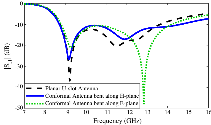
Figure 2. Comparison of the reflection coefficients of the planar and conformal U-slot patch antennas bent along the E - and H -planes, when h = 3.175 \text{ mm} , \alpha = 100^\circ , and r = 15 \text{ mm} .
