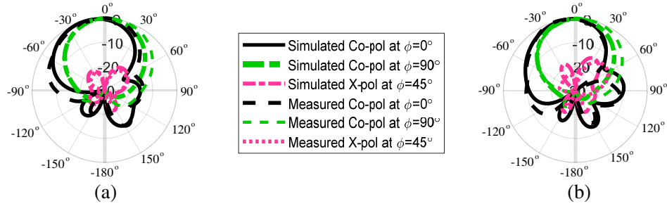
Figure 7. Measured and simulated co-polar radiation patterns at the principal planes and cross-pol radiation patterns at the \phi = 45^\circ plane (a) 9.5 GHz and (b) 11.5 GHz.
