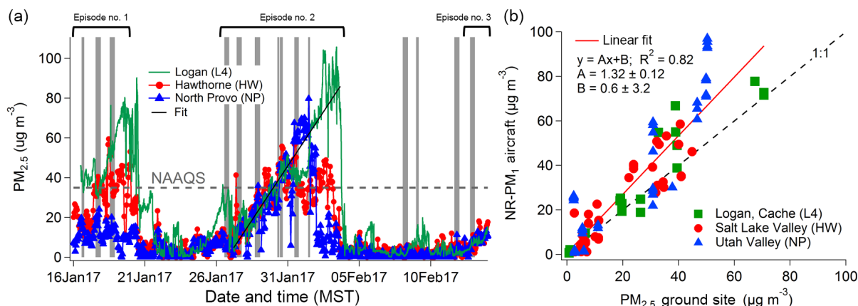
Figure 2. \text{PM}_{2.5} measurements from three ground sites during UWFPS. (a) Time series of \text{PM}_{2.5} measured in Logan (L4), Cache Valley, in green; at Hawthorne Elementary School (HW), Salt Lake Valley, in red; and in North Provo (NP), Utah Valley, in blue. The grey shaded areas correspond to the times of Twin Otter flights; the horizontal dashed line indicates the National Ambient Air Quality Standard (NAAQS) of 35 \mu\text{g m}^{-3} for 24 h averaged \text{PM}_{2.5} . The black solid line is a fit over all the data of the increase in \text{PM}_{2.5} during Episode 2. The slope is 10.89 \pm 0.08 \mu\text{g m}^{-3} \text{ day}^{-1} (slope \pm 95\% CI). (b) Comparison of the non-refractory (NR) \text{PM}_1 measured with the AMS from the Twin Otter for altitudes lower than 50 m a.g.l. during the missed approaches at the airports closest to the ground site measurements. The dashed line is the 1 : 1 line and the red solid line is a linear fit; correlation coefficient, fit coefficients, and their 95 % CI are reported in the legend.
