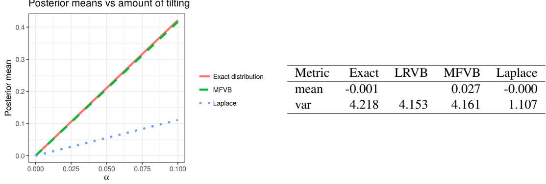
Figure 4: Effect of tilting on a univariate over-dispersed distribution.
