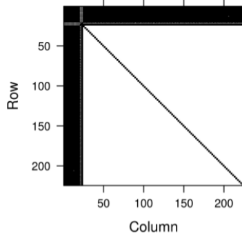
Figure 12: Sparsity pattern of top-left sub-matrix of \mathbf{H}_{\eta\eta} for the logit GLMM model. The axis numbers represent indices within \eta , and black indicates non-zero entries of \mathbf{H}_{\eta\eta} .
