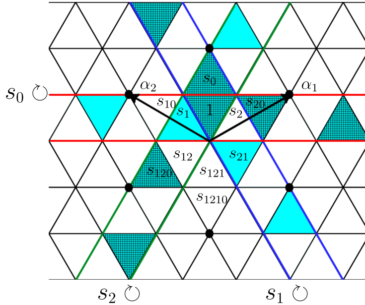
Figure 3: The elements of \tilde{S}_3^P for the parabolic P corresponding to Gr(1, 3) are colored blue. The shaded blue alcoves are the elements of \tilde{S}_3^P \cap \tilde{S}_3^0 , which are also minimal length coset representatives.
