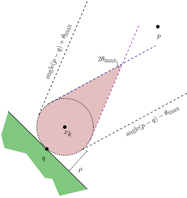
Fig. 5. Point p is too far from the boundary to be certainly covered by any plan under our robot model. See Theorem 2.
