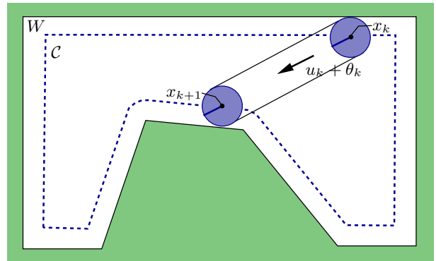
Fig. 2. An illustration of the basic notation. At stage k , the robot moves in direction u_k + \theta_k , from x_k to x_{k+1} , covering a portion of the environment W along the way. Both x_k and x_{k+1} are points along the boundary of C . However, the robot does not necessarily know x_k , and certainly does not know \theta_k .
