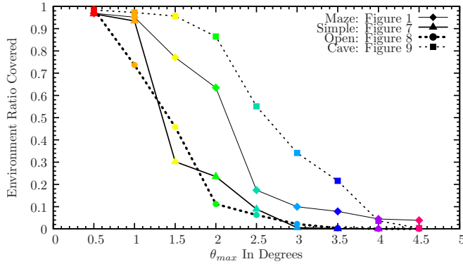
Fig. 10. A plot comparing the ratio of each environment the algorithm can guarantee to cover as accuracy degrades when \theta_{\max} is allowed to grow.
