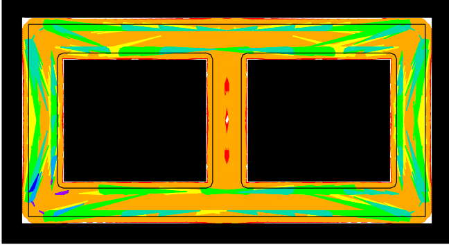
Fig. 7. A simple environment with two large holes. The robot began in the lower left corner and became stuck there as \theta_{\max} reached 3 degrees (■).
