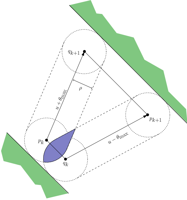
Fig. 4. Computing the CCR for a single safe action, as described in Theorem 1.
