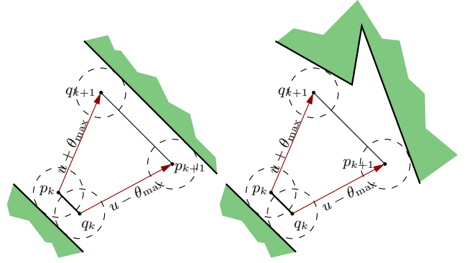
Fig. 3. [left] An example of a safe action. [right] This action is unsafe, because p_{k+1} and q_{k+1} lie on different edges of the boundary.
