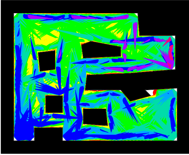
Fig. 9. A more natural cave-like environment. As error grew, the robot retained the ability to navigate around most of the environment until \theta_{\max} reached 4 degrees (■), but lost the ability to cover the more spacious open areas past 2 degrees (■). This environment demonstrates the method's ability to deal with non-uniform features.
