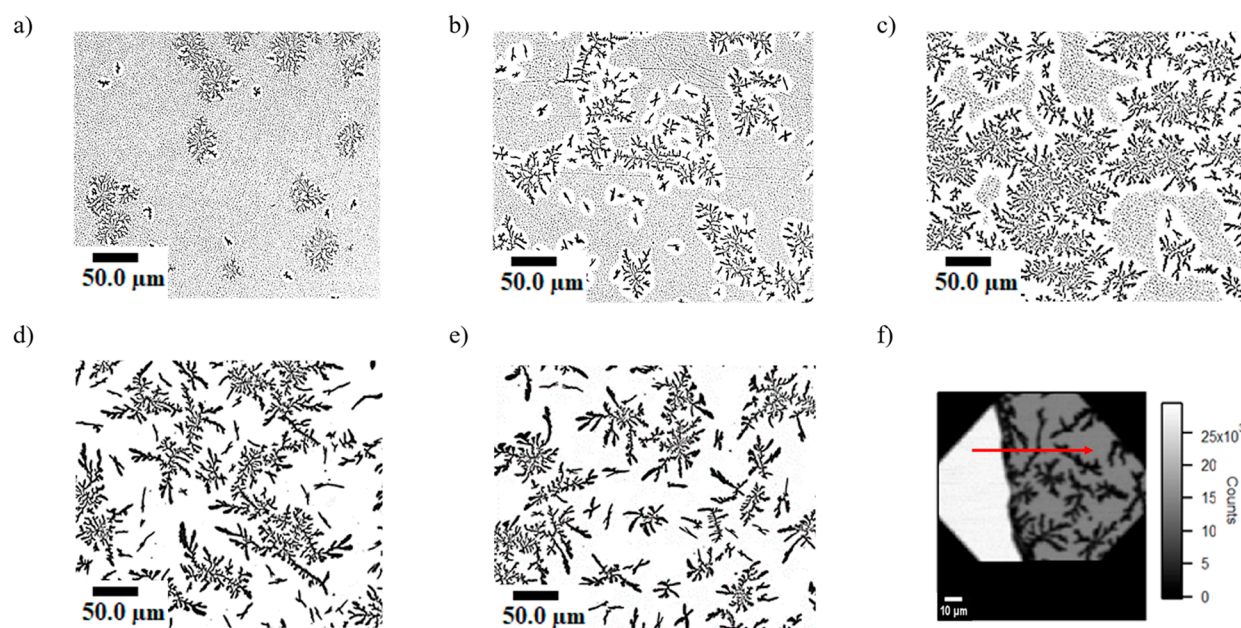
Figure 3. Transmission VLM images of phase-separated blends of a 6:4 (w/w) PffBT4T- C_9C_{13} :PC _{71} BM annealed at 240 °C for (a) 5 min, (b) 15 min, (c) 30 min, (d) 23 h, and (e) 80 h. PCBM depletion regions are observed to be the small areas beside the PCBM crystals as shown in panel a and then they grow with annealing time displayed in panels b and c until they are expanded to the whole region in panels d and e. (f) 2D STXM image of 6:4 (w/w) PffBT4T- C_9C_{13} :PC _{71} BM blend annealed at 200 °C for 3 days and the red arrow indicates the location and direction of STXM line scan. The uniform white area is a region without sample that is used to measure the incident X-ray intensity.
