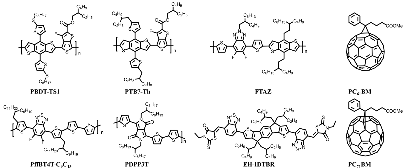
Figure 2. Molecular structures of materials used.
