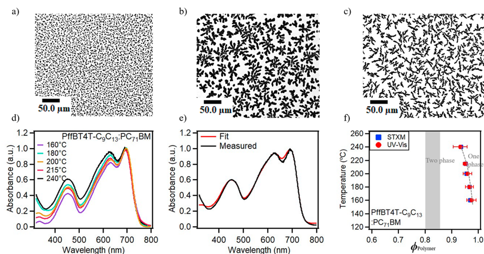
Figure 4. Transmission VLM images of phase-separated blends of 1:1 (w/w) PffBT4T- C_9C_{13} :PC _{71} BM annealed at (a) 160 °C for 78 h, (b) 180 °C for 65 h, and (c) 200 °C for 78 h. (d) UV-vis absorption spectra of 1:1 (w/w) PffBT4T- C_9C_{13} :PC _{71} BM blends annealed at different temperatures and the highest intensity of each spectrum is normalized to be 1. (e) Comparison between the fitted spectrum from UV-vis method and the measured spectrum for 1:1 (w/w) PffBT4T- C_9C_{13} :PC _{71} BM blend annealed at 240 °C. (f) The plot of temperature dependent uncorrected liquidus miscibility for PffBT4T- C_9C_{13} mixed with PC _{71} BM, where \phi_{\text{polymer}} is the uncorrected composition of PffBT4T- C_9C_{13} in the amorphous, mixed phase. It is determined by both the UV-vis method and STXM. The gray band is the reported percolation threshold, 8 where the polymer volume fraction is around 0.8–0.85. The liquidus line separating one phase and two phase regions are conceptual and not fits to a model or theory.
