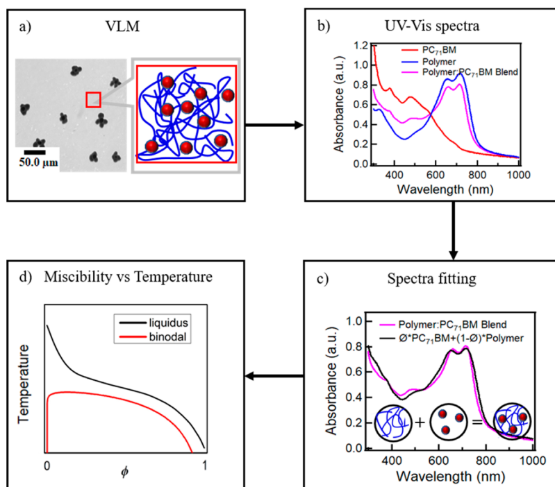
Figure 1. A flowchart describing the steps to measure the temperature-dependent miscibility. Take a polymer:PC 71 BM system as an example. (a) Use of visible light microscopy (VLM) to ensure the local thermodynamic equilibrium is reached. This local thermodynamic equilibrium state is reached in a thermally annealed polymer:fullerene blend film, when the fullerene crystals are embedded in a uniform matrix without depletion gradients. (b) UV–vis absorption spectra are acquired on the neat films and thermally annealed blend films. (c) The polymer:fullerene blend spectrum is fitted with the linear combination of the neat, mass–thickness normalized reference spectra. (d) The liquidus line can be acquired. In the phase diagram, the liquidus is the equilibrium composition between the amorphous, mixed phase and the PCBM crystals corresponding to the liquidus miscibility while the binodal is the coexistence curve of binary amorphous mixtures of polymer:PCBM blends corresponding to the amorphous miscibility when PCBM crystals have been suppressed. We note that the UV–vis averages over both the polymer-rich matrix as well as the PCBM crystals. We will show later that the presence of PCBM crystals does not introduce a significant measurement error, as the PCBM crystals are so thick and absorbing that they act similar to any completely opaque “dust spec” and thus do not contribute significantly to the UV–vis spectrum or a heterogeneous sample measured in absorption by detecting transmitted light.
