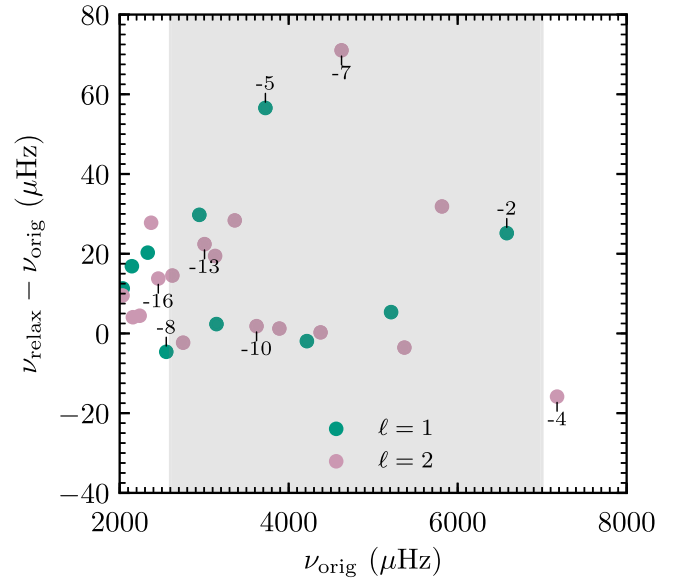
Figure 3. Differences between the adiabatic frequencies \nu of \ell = 1 and \ell = 2 g-modes in the relaxed and original MESA models. Selected modes are labeled by their radial order \tilde{n} . The shaded region marks the range of frequencies seen in the Kepler observations of KIC 08626021.
