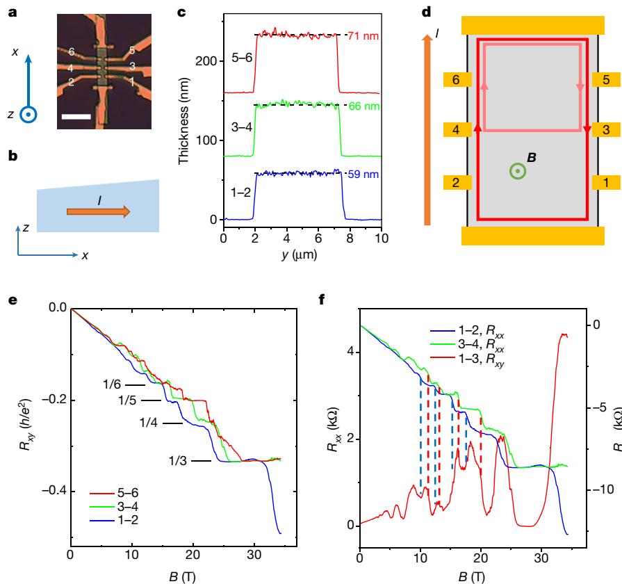
Fig. 2 | Quantum Hall effect in sample 1, which is wedge-shaped along the x axis. a , Optical image of the Hall bar device with terminals indexed. Scale bar, 15 \mu\text{m} . b , Schematic of the sample geometry. The sample thickness increases slightly along the x axis. The electric current I is applied along the x axis. c , Cross-sectional thickness profiles (offset for clarity) determined using atomic force microscopy near the three pairs of Hall electrodes (1–2, 3–4 and 5–6). The root-mean-square roughness in the thickness is roughly 2.0–2.6 nm. d , Schematic of the quantum Hall edge states for the wedge-shaped sample with a thickness gradient along the x axis. The electrodes are marked by the yellow boxes with the current I along the x direction. The light and dark red curves
