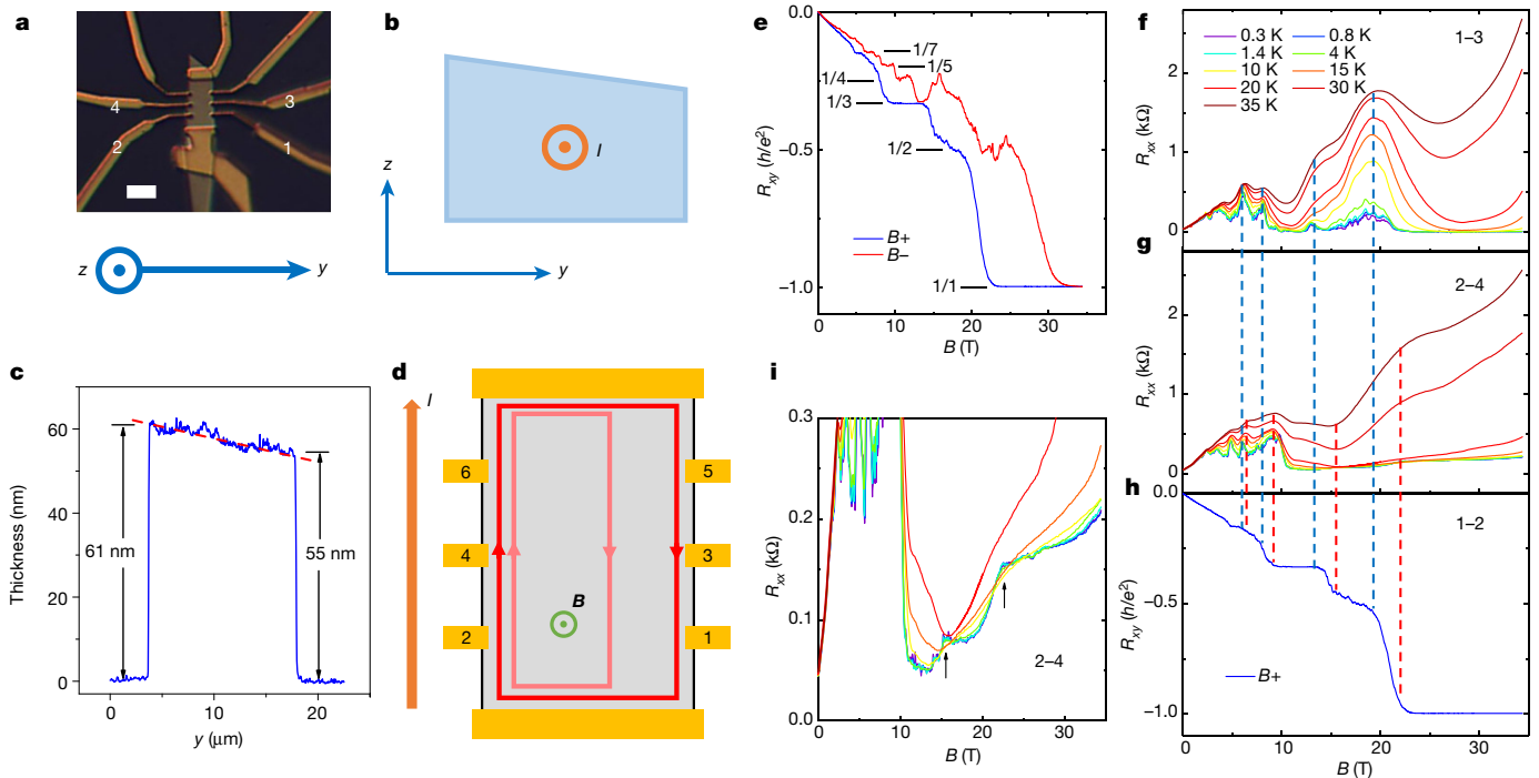
Fig. 3 | Quantum Hall effect in sample 2, which is wedge-shaped along the y axis. a , Optical image of the Hall bar device with terminals indexed. Scale bar, 15 \mu\text{m} . b , Schematic of the sample geometry. The sample thickness slightly increases along the y axis. c , Cross-sectional thickness profiles across the sample along the y axis. The red dashed line highlights the trend of the thickness variation. d , Schematic of the quantum Hall edge states for the wedge-shaped sample with a thickness gradient along the y axis. e , Hall resistance R_{xy} measured with the magnetic field along the positive ( B+ ) and negative ( B- ) z directions. The values of R_{xy} at the
