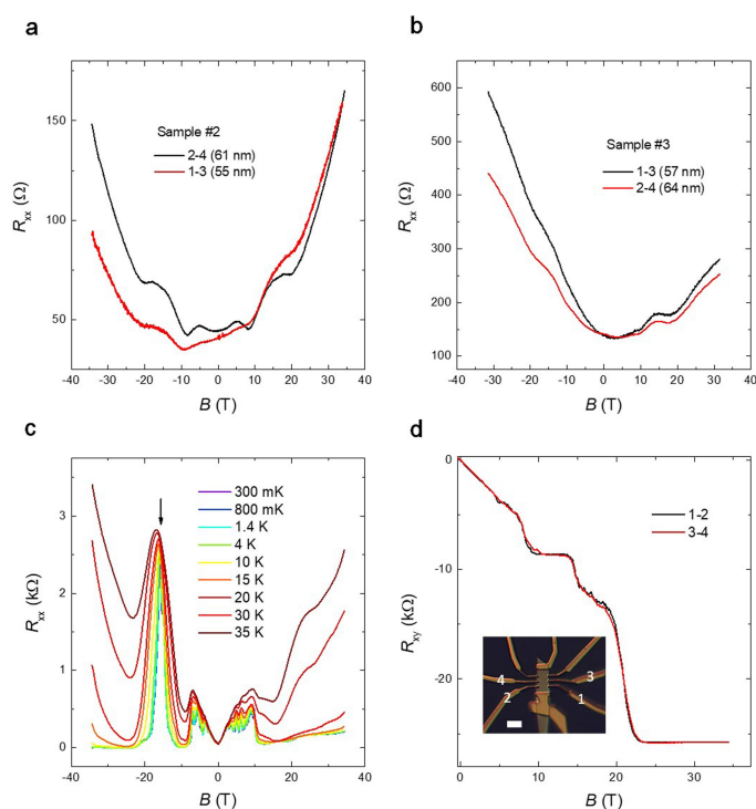
Extended Data Fig. 7 | Additional transport data for samples 2 and 3.
