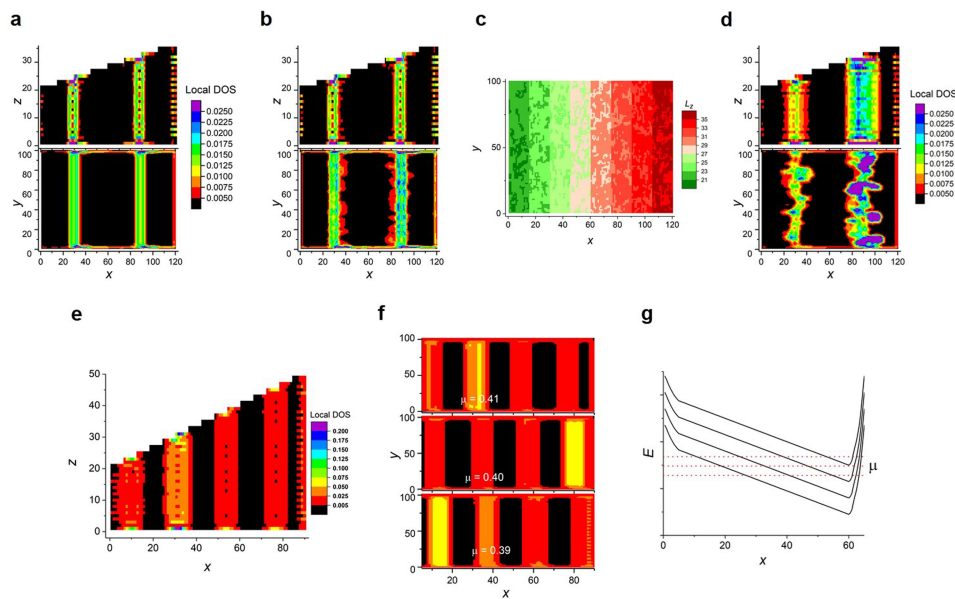
Extended Data Fig. 1 | Numerical simulations of a wedge-shaped Weyl semimetal. a, b, The local density of states (DOS; colour scale) in different cross-sections of a clean system with random impurities W = 0 ( a ) and a system with random impurities W = 0.1 (both in the bulk and on the surface; b ), showing the location and extent of the modes. The system size is L_x = 120 , L_y = 100 and L_z \in [21, 35] , with sharp side walls at both ends. The upper panels show trapezoidal x - z cross-sections, with the local DOS averaged across y \in [0.1L_y, 0.9L_y] to exclude contributions from the modes on the side walls at both ends in the y direction. The lower panels show the x - y cross-sections, with the local DOS averaged across the thickness L_z . We set the Fermi energy to \mu = 0.4 . c, d, Real-space
