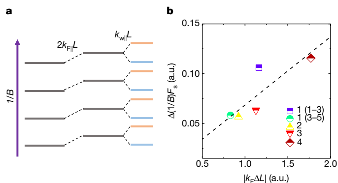
Fig. 5 | Analysis of the Landau-level shift in Weyl orbits. a , Schematic of the Landau-level shift process. The first transition corresponds to the global phase shift from k_{F\parallel} , which is independent of the chirality. The second transition (or splitting) corresponds to the phase shift from k_{w\parallel} , which splits the Shubnikov-de Haas oscillations from the two sets of degenerate Weyl orbits in \text{Cd}_3\text{As}_2 . L is the sample thickness. b , Quantitative analysis of the global phase shift \Delta(1/B) in several samples. \Delta L is the thickness variation. The overall trend follows a simple linear relationship (dashed line). a.u., arbitrary units.
