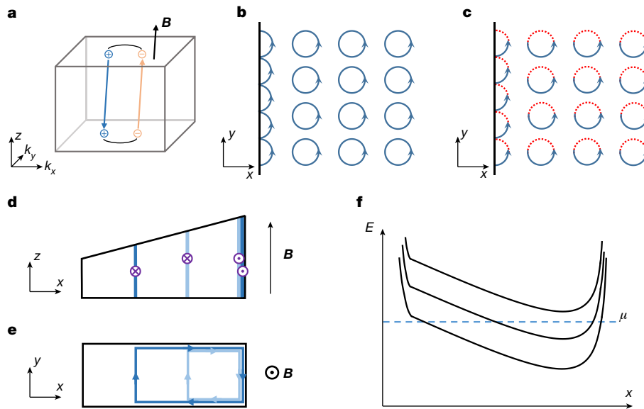
Fig. 1 | The quantum Hall effect in Weyl orbits. a , Illustration of the Weyl orbit under magnetic field B . Two pairs of Weyl nodes of opposite chirality (+ and −) in the bulk are connected by Fermi arcs (black arcs) on two surfaces in the k_x – k_y plane. Electrons propagate between the two surfaces (blue and orange arrows) in real space along the z direction via the chiral Landau levels to complete the cyclotron motion. b , Cyclotron quantum Hall orbits of a 2D electron liquid in a magnetic field perpendicular to the x – y plane. The chiral mode forms along the edge (left). c , Weyl orbits, which consist of surface Fermi arcs and bulk chiral Landau levels of a 3D Weyl semimetal in a magnetic field perpendicular to the x – y plane. The solid blue and dashed red trajectories correspond to Fermi arcs on the top and bottom surfaces, respectively, which are connected through the chiral Landau levels in the bulk. d , A geometry with varying thickness z along
