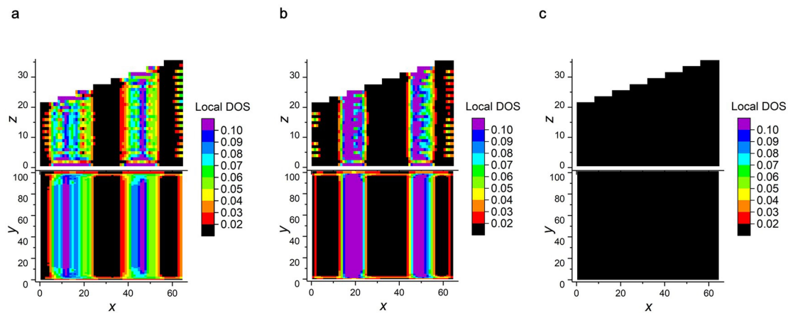
Extended Data Fig. 3 | Numerical simulations of a wedge-shaped Dirac semimetal. a–c , Local DOS (colour scale) of Dirac semimetal models showing the location and extent of the modes for different orbit hybridization amplitudes: \Delta = 0.1 in the two surface layers at the top and bottom surfaces ( a ); \Delta = 0.05 throughout the entire bulk ( b ); and \Delta = 0.2 ( c ). The system size is L_x = 64 , L_y = 100 and L_z \in [21, 35] , with sharp side
