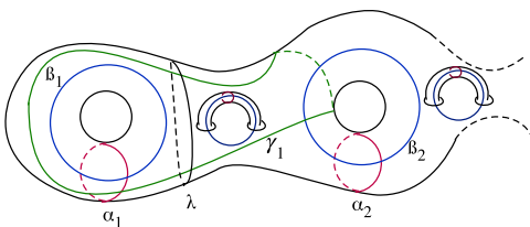
Fig. 6. \alpha_1 \mathcal{D} \beta_1, \gamma_1 \mathcal{D} \alpha_1 .
