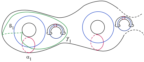
Fig. 5. \alpha_1 \mathcal{D} \beta_1 \mathcal{D} \gamma_1 \mathcal{D} \alpha_1 .
