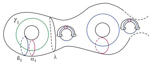
Fig. 4. \alpha_1 \mathcal{P} \beta_1 \mathcal{D} \gamma_1 .
