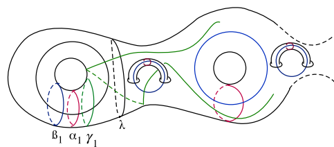
Fig. 3. \alpha_1 \mathcal{P} \beta_1 \mathcal{P} \gamma_1 .
