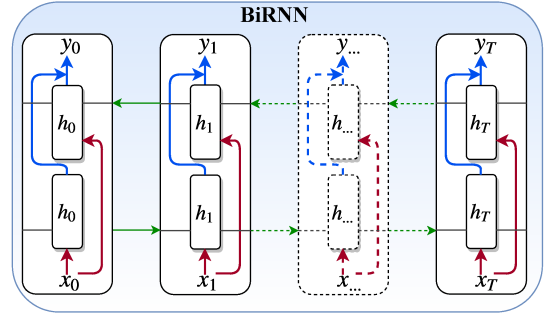
Figure 3: A schematic diagram of the bidirectional recurrent neural network.
