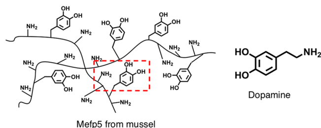
Figure 7. Schematic illustration of Mefp-5 protein from mussels and dopamine-containing amine and catechol functional groups (broken red square) used to design mussel-inspired surface coatings. 100
