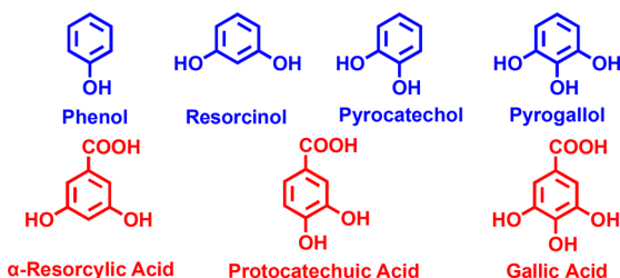
Figure 5. Natural plant phenols, polyphenols, and constitutional isomeric AB 2 and AB 3 phenolic acids.
