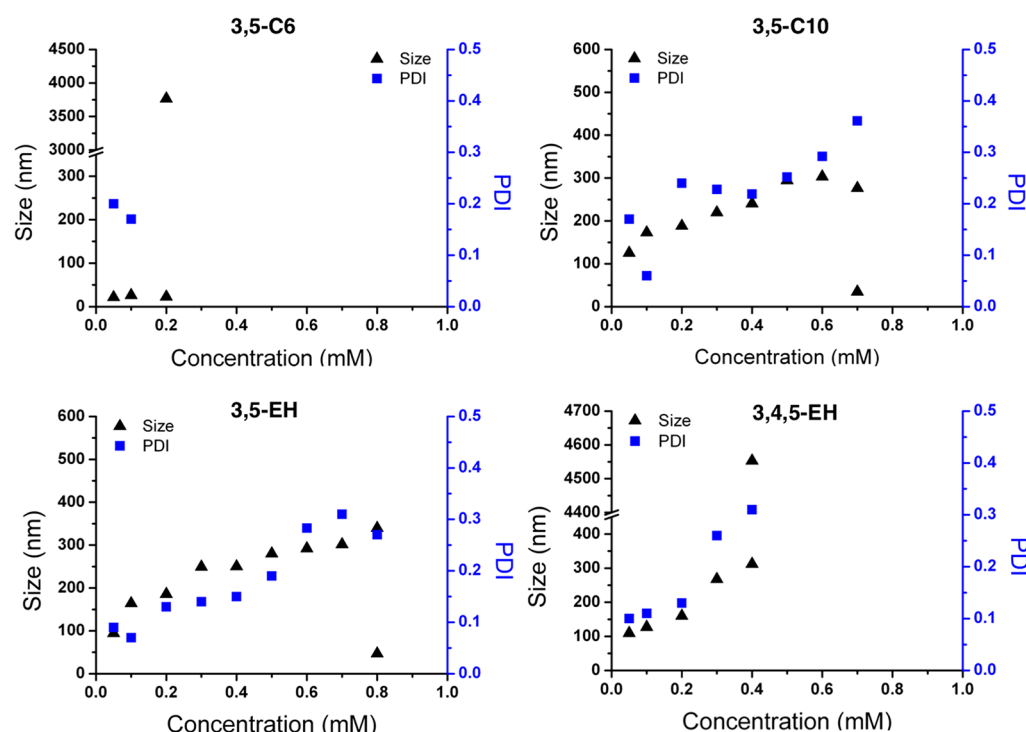
Figure 9. Representative concentration-dependent dynamic light scattering data.
