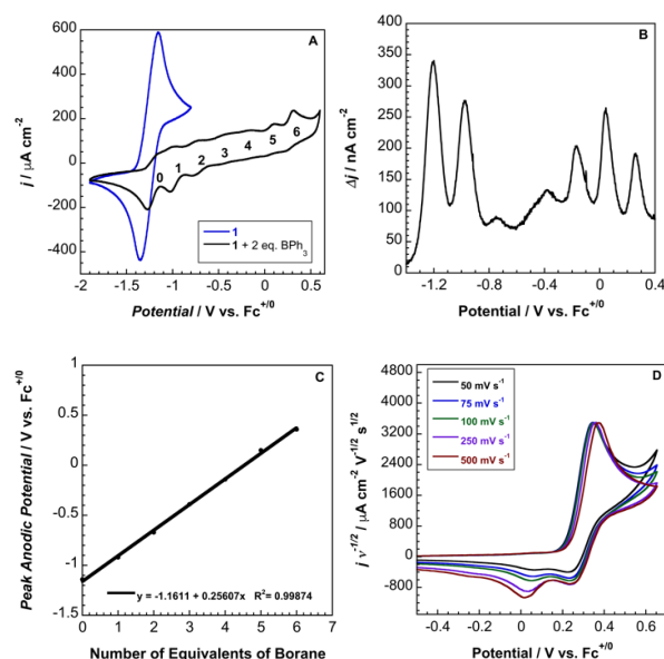
Figure 4. A. Cyclic voltammograms of 5 mM 1b (blue) and 5 mM 1b with two equivalents of BPh_3 (black) at 100\text{ mV s}^{-1} in DCM with 0.1 M TBAPF_6 . B. Differential pulse voltammetry of 1b with two equivalents of BPh_3 . C. Linear regression of peak anodic potential from cyclic voltammetry versus number of BPh_3 molecules coordinated to ferrocyanide. D. Normalized scan-rate dependence of 2 in MeCN with 0.2 M TBAPF_6 .
