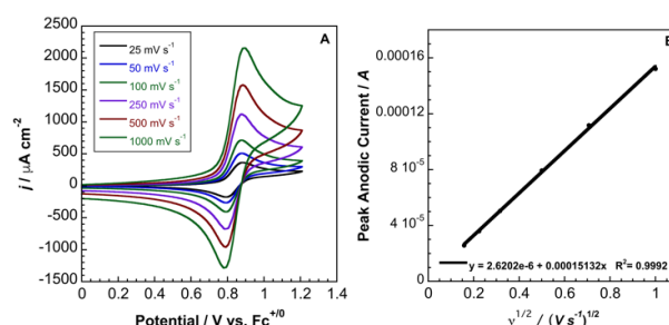
Figure 5. A. Cyclic voltammetry (scan rates from 25\text{ mV s}^{-1} to 1000\text{ mV s}^{-1} ) of 3.6 mM 3 in acetonitrile with 0.2 M TBAPF_6 . Potentials relative to Fc^{+/0} . B. Randles-Sevcik plot of the CV data from 5A.
