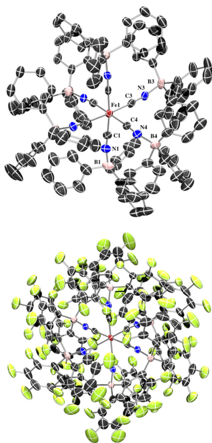
Figure 1. A. Molecular structure of (\text{TEA})_4[\text{Fe}(\text{CN-BPh}_3)_6] ( 2 ). Thermal ellipsoids set at 50% probability. Cations and protons omitted for clarity. Selected bond distances and angles: Fe1-C1: 1.908(7) Å, Fe1-C3: 1.913(8) Å, Fe1-C4: 1.908(8) Å, C1-N1: 1.170(9) Å, C3-N3: 1.164(10) Å, C4-N4: 1.166(10) Å, N1-B1: 1.559(9) Å, N3-B3: 1.573(10) Å, N4-B4: 1.557(10) Å, Fe1-C1-N1: 174.0(7)°, Fe1-C3-N3: 174.0(7)°, Fe1-C4-N4: 179.6(8)°, C1-N1-B1: 172.0(8)°, C3-N3-B3: 173.5(8)°, C4-N4-B4: 176.3(7)°. B. Molecular structure of (\text{PPN})_4[\text{Fe}(\text{CN-B}(\text{C}_6\text{F}_5)_3)_6] ( 3 ). Thermal ellipsoids set at 50% probability. Cations omitted for clarity. Selected bond distances and angles (labels as in 2 ): Fe1-C1: 1.899(4) Å, Fe1-C3: 1.904(3) Å, Fe1-C4: 1.897(3) Å, C1-N1: 1.146(4) Å, C3-N3: 1.152(4) Å, C4-N4: 1.160(4) Å, N1-B1: 1.545(5) Å, N3-B3: 1.550(5) Å, N4-B4: 1.551(4) Å, Fe1-C1-N1: 176.9(3)°, Fe1-C3-N3: 177.9(3)°, Fe1-C4-N4: 175.9(3)°, C1-N1-B1: 173.2(3)°, C3-N3-B3: 175.1(3)°, C4-N4-B4: 173.3(4)°.
