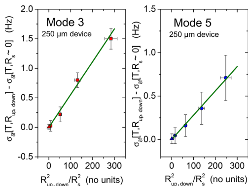
Figure 7. Universal plot for modes 3 and 5. Normalized frequency noise plot for the same 250 \mu\text{m} device, for modes n = 3 (left) and n = 5 (right). The lines are linear fits (see text).
