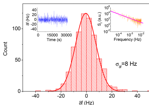
Figure 5. Large-amplitude statistics. Similar graphs to those in Figure 4 were obtained on the upper bifurcation point f_{\text{up}} (frequency jumps time trace in the left inset, power spectrum of frequency in the right inset, and histogram of \delta f in the main part of the graph). The line is a Gaussian fit, while the power spectrum follows 1/f^{1+\epsilon} (see text).
