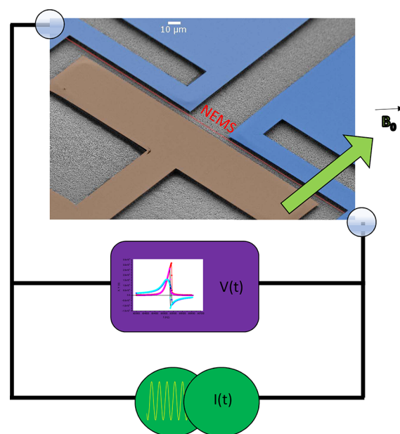
Figure 1. Device and setup. SEM image of the 250 \mu\text{m} device measured in this work. The gate electrode (brown) is not used here. The actual NEMS device is the red-colored string in between the two (light blue) electrodes. The lock-in detector (violet), magnetic field, and drive generator (in green) are also depicted in a schematic fashion to illustrate the magnetomotive technique.
