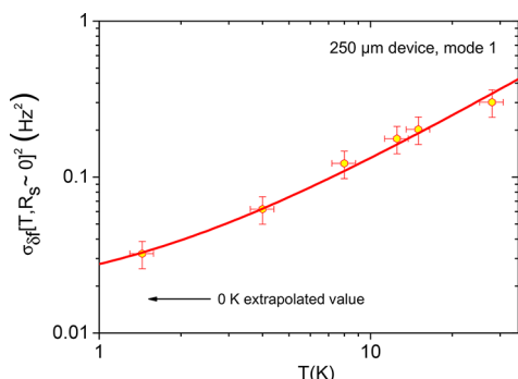
Figure 8. Temperature dependence of frequency fluctuations. Allan variance \sigma_{\delta f}^2 as a function of temperature (first mode of 250\ \mu\text{m} device), as obtained for small motion R \rightarrow R_s \approx 0 . The line is a linear fit, with the T_0 = 0\ \text{K} extrapolated value emphasized by the arrow (see text). The variance of damping fluctuations \sigma_{\delta \Delta f}^2 is constant in the same range of temperatures.
