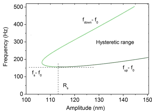
Figure 3. Bifurcation branches. Calculated bifurcation frequencies from eqs 1 and 2 for the 250 \mu\text{m} device and magnetototively loaded Q of 5000 (1 T field).
