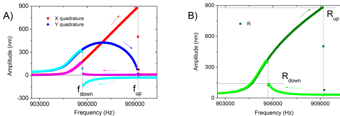
Figure 2. Nonlinear (Duffing) resonance. (A) Duffing resonance line (X and Y quadratures) measured on the 250 \mu\text{m} device at 4.2 K under vacuum, for a drive force of 81 pN, in a 1 T field. The directions of frequency sweeps are depicted by arrows. Vertical dashed lines indicate the two bifurcation points f_{\text{up,down}} . (B) Amplitude R = \sqrt{X^2 + Y^2} corresponding to A. Bifurcation points are indicated with their amplitudes R_{\text{up,down}} .
