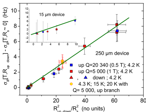
Figure 6. Universal plot for mode 1. Frequency noise increase vs squared amplitude normalized to the spinodal value R_s , for the first mode n = 1 of the 250 \mu\text{m} device. Various T_0 and B_0 (hence Q ) have been used (see legend). Squares stand for upper branch bifurcation; triangles for lower. Inset: same result obtained with a 15 \mu\text{m} beam having \beta = 1.1 \times 10^{19} Hz/m 2 (4.2 K and Q = 17\,000 red squares; 800 mK and Q = 31\,000 blue dots; the magnetomotive field broadening was negligible). The green line is a linear fit (see text).
