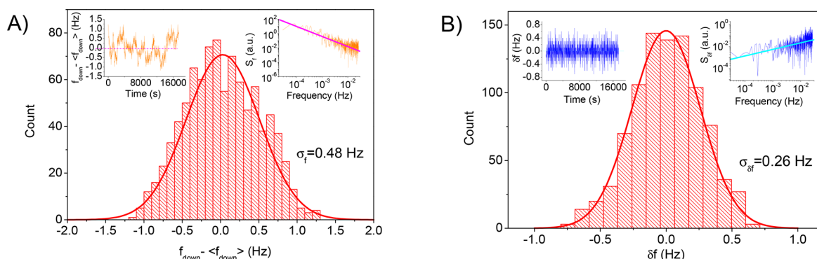
Figure 4. Statistics on frequency at low amplitudes. (A) Histogram obtained on the f_{\text{down}} relaxation point of Figure 2 (left inset: actual frequency time trace; right inset: power spectrum of the frequency fluctuations, displaying 1/f -type structure). (B) Histogram obtained on the frequency jumps \delta f computed from the f_{\text{down}} time trace (left inset: \delta f time trace; right inset: power spectrum). The lines are Gaussian fits, and the power-law dependencies of the spectra are discussed in the text.
