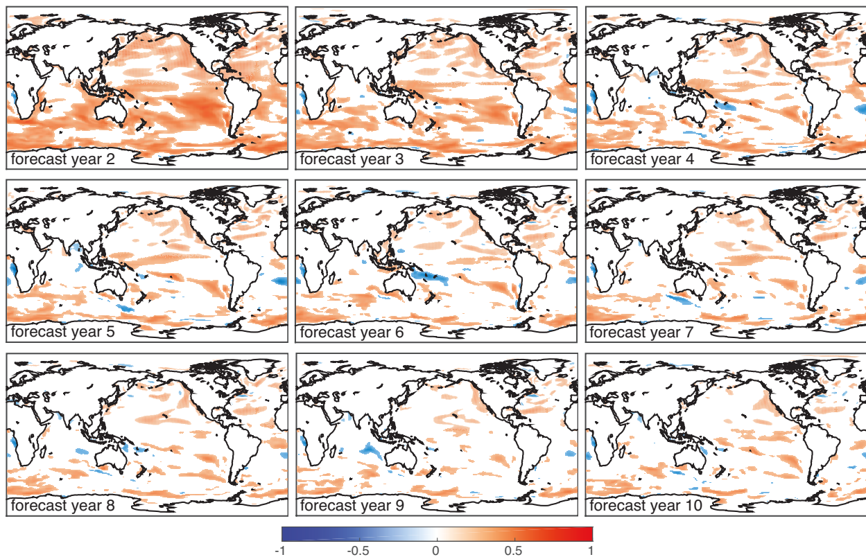
Figure S1. Predictability of air-sea CO 2 flux, as indicated by the correlation coefficient of detrended, air-sea CO 2 flux anomalies from the CISM-DPLE initialized forecast for a range of lead years with the reconstruction. Correlation coefficients that are not statistically significant at the 95% level using a t test are assigned a value of zero.
