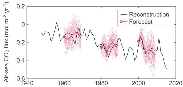
Figure 1. Annual mean air–sea \text{CO}_2 flux ( \text{mol m}^{-2} \text{yr}^{-1} ) in the South Pacific subtropical permanently stratified biome for the (black) model reconstruction and (pink) CESM-DPLE decadal forecasts initiated in 1960, 1980, and 2000 (other forecasts omitted for visual clarity). The thick magenta line represents the ensemble mean forecast; open circles show the ensemble mean in forecast year 1. Positive fluxes denote ocean outgassing. Forecasts have been drift-corrected and adjusted to match the reconstruction climatological mean for ease of visual comparison.
