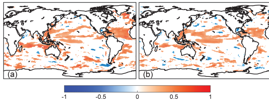
Figure 7. Air–sea \text{CO}_2 flux predictive skill, as indicated by the correlation coefficient of air–sea \text{CO}_2 flux (a) anomalies, and (b) linearly detrended anomalies from the CESM-DPLE initialized forecast in year 1 with the Landschützer et al. (2016) observational product over 1995–2015. Correlation coefficients that are not statistically significant at the 95 % level using a t test are assigned a value of zero.
