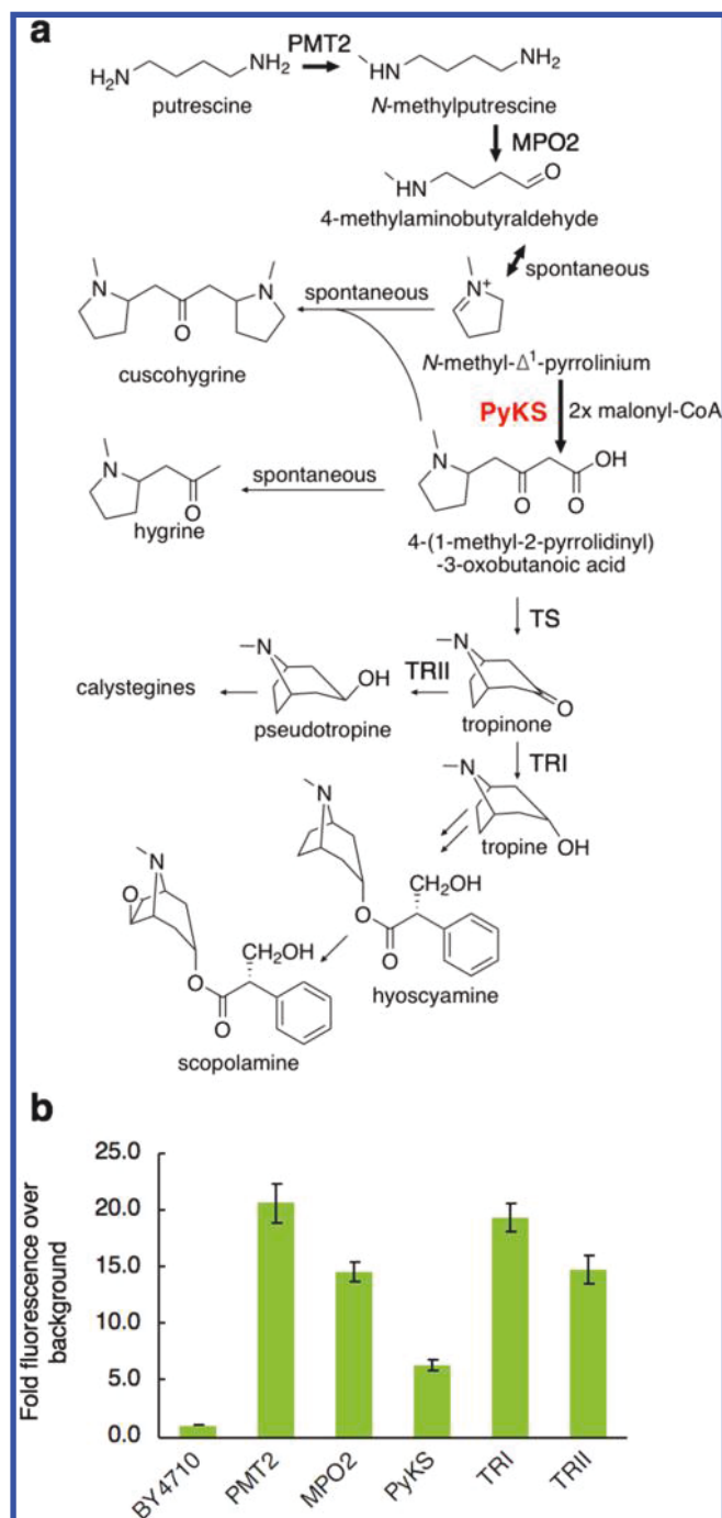
Figure 1. Tropane alkaloids (TA) pathway from Atropa belladonna (Ab). (a) The conversion of putrescine to N -methylputrescine by PMT2 is the first committed step in TA biosynthesis. The enzyme engineered for improved solubility in this work, PyKS, performs two rounds of ketide synthase (Claisen condensation) activity on N -methyl- \Delta^1 -pyrrolinium with two units of malonyl-CoA to form 4-(1-methyl-2-pyrrolidinyl)-3-oxobutanoic acid. Hyoscyamine and scopolamine are medically relevant small molecules. (b) Expression yield of Ab genes in yeast via GFP-tagging confirms poor heterologous expression of PyKS. Fluorescence of S. cerevisiae strain BY4710 cells expressing GFP-tagged Ab genes under galactose induction was quantified using flow cytometry. Error bars represent one standard deviation of at least three independent measurements.
