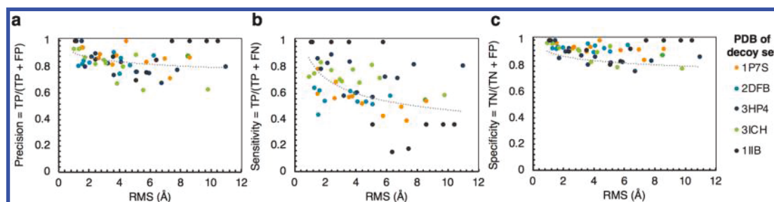
Figure 4. Automated generation of filter-passing mutations with a PyRosetta script is robust for use on predicted structural models. Precision (a), sensitivity (b), and specificity (c) were calculated by comparing the results of running our PyRosetta mutation filtering script on five different PDB crystal structures and their corresponding decoy sets (see methods).
