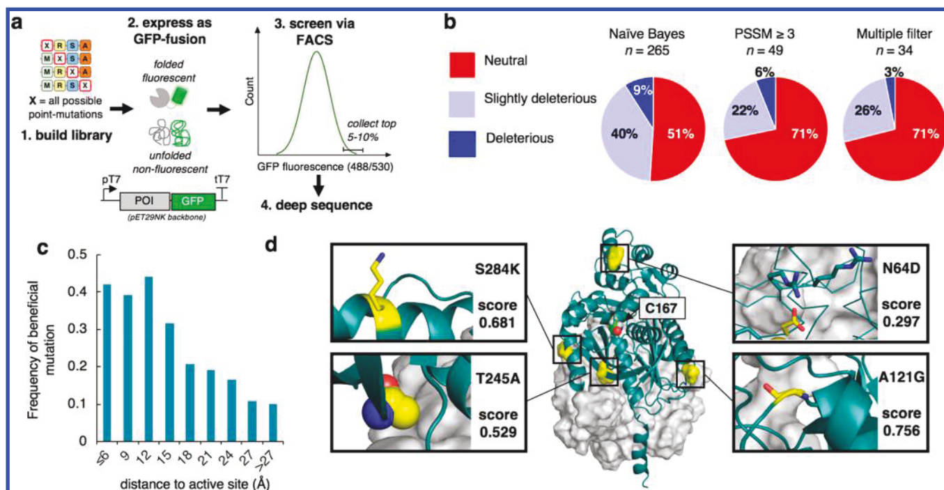
Figure 2. Deep mutational scanning using GFP-fusion solubility screen and filtering to identify catalytically neutral stabilizing mutations. (a) Method overview. A comprehensive site-saturation library for a protein of interest (POI) is generated using nicking mutagenesis (1). The POI is genetically encoded as an N-terminal fusion to GFP (2), where upon expression folded POIs will permit the folding and subsequent chromophore formation of GFP, while unfolded protein will be nonfluorescent. The amount of folded fusion protein per cell correlates with solubility/stability of the POI variant. The library is expressed in E. coli and screened for GFP fluorescence using FACS (3), and the resulting pre- and postscreening libraries are deep sequenced (4). (b) Results from applying various filtering strategies to the levoglucosan kinase (LGK) GFP-fusion and fitness selections data sets. The best strategy "Multiple filter" includes distance to active site ( 15 \geq \text{\AA} ), PSSM ( \geq 0 ), contact number ( \leq 16 ), and exclusion of mutations to/from proline. (c) The frequency of beneficial (solubility-enhancing) mutations of PyKS identified from the GFP-fusion experiment as a function of distance to catalytic active site. (d) Structural analysis of high solubility score mutations indicates that many improve surface charge characteristics (S284K, N64D), hydrophobic core packing (T245A), and secondary structural elements like loops (A121G). The gray surface representation is the dimer subunit. C167 is the putative catalytic nucleophile.
