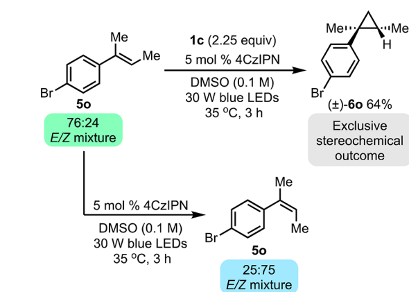
Scheme 3. Stereoconvergent Cyclopropanation
