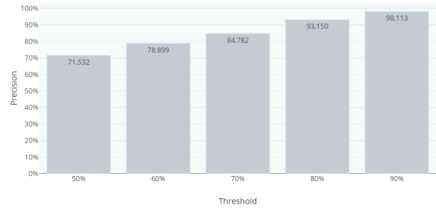
Fig. 4. Precision vs. Discrimination Threshold: Trial 4
