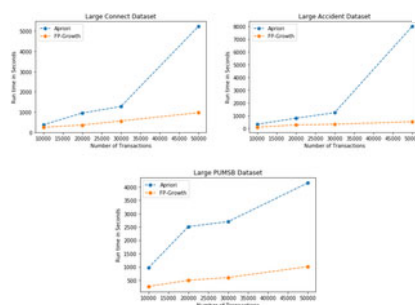
Fig 6. Experimental results on large datasets.
