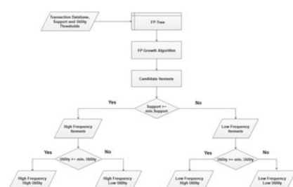
Fig 1. Phase 1—Proposed method.
