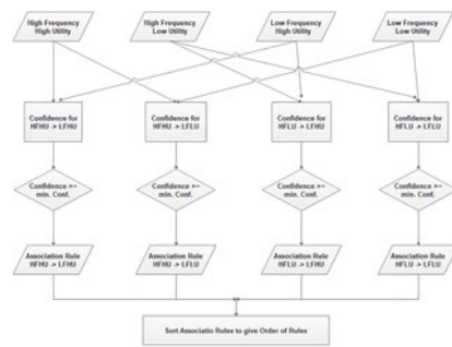
Fig 2. Phase 2—Proposed method.
