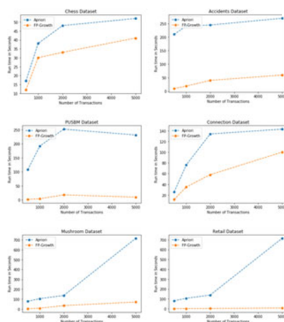
Fig 5. Experimental results on small datasets.
